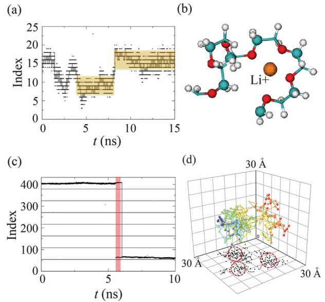
FIG. 3 (color). (a) Index of oxygen atoms of a PEO chain interacting with a \text{Li}^+ ion at time t , representing the intrachain hopping process. Gray line is an average at each time. Shaded areas indicate cages formed at different times. (b) Snapshot of MD simulation showing a \text{Li}^+ caged by a PEO chain. (c) Index of oxygen atoms from all oxygens in the simulation box interacting with a \text{Li}^+ ion at time t , representing an interchain hopping process. The gray vertical line at 6 ns indicates the moment of completed transition from one cage to another cage of different PEO chains. Shaded area indicates the transition time of less than 1 ns. (d) \text{Li}^+ trajectory plotted every 100 ps during 30 ns. Projected coordinates are shown in the x - y plane to help with visualization. Higher density of coordinate points indicates \text{Li}^+ trapped in the cage of oxygens (dashed red circles).
