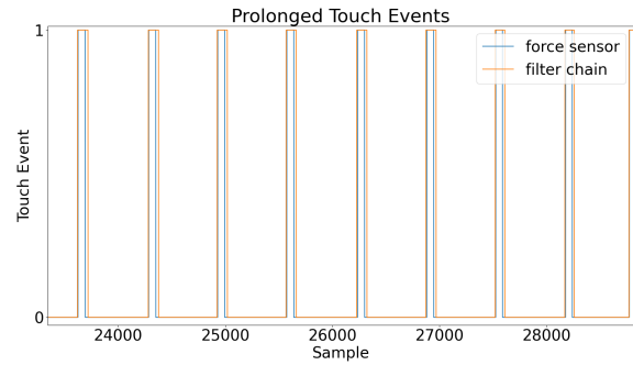
Figure 6: Example of prolonged touch events due to a low pass filter (on the EMC data).
