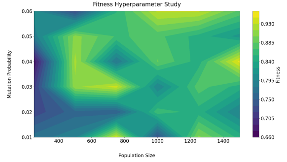
Figure 3: Fitness values on the test dataset for tournament k = 30 .
