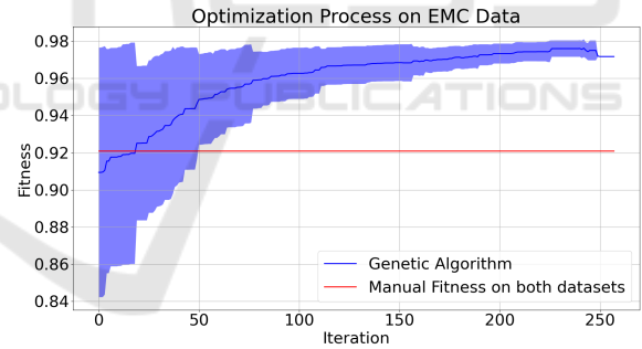
Figure 5: Learning Process of the GA plus minus standard deviation on the EMC data. The plot further contains the fitness of the manual calibration on both the training and validation dataset.
