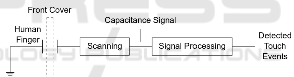
Figure 1: Working principle of a capacitive touch device.
