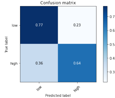
Fig. 2. Confusion matrix of the neural network for the recognition of low and high conversational engagement (test set).
