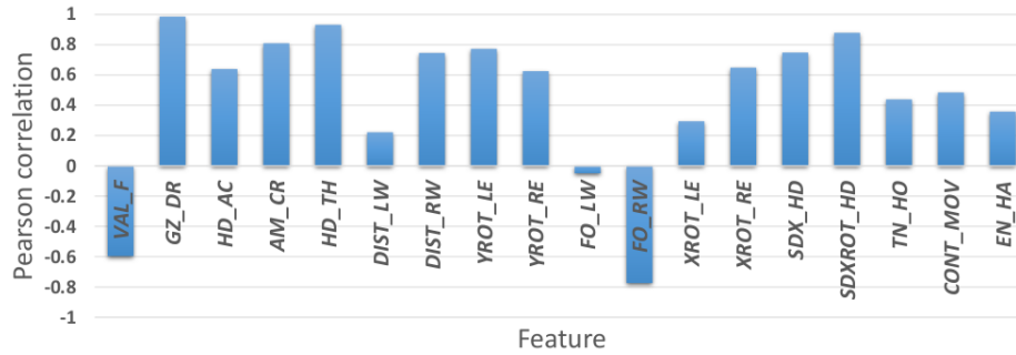
Fig. 4. Pearson correlation between the absolute change of the feature values and the LIME classification relevance scores for every feature. The features are from left to right: Valence Face , Gaze behavior , Head activity , Arms crossed , Head touch , X distance of left/right wrist and hip , Y rotation left/right elbow , Y distance of left/right wrist and hip , X rotation left/right elbow , Standard deviation head movement in X axis , Standard deviation Head X rotation , Turn hold , Continuous movement , Gesticulation .
