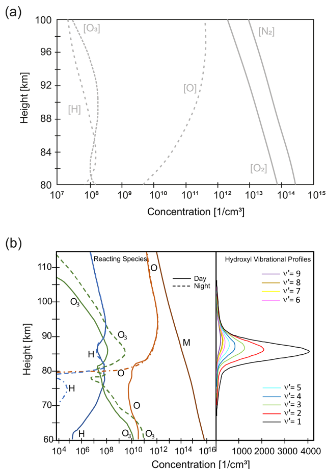
Figure 1. (a) Number density of the two major ( \text{O}_2 and \text{N}_2 , solid lines) and the three minor ( \text{O}_3 , \text{O} , and \text{H} , dashed lines) species involved in the production of \text{OH}^* between 80 and 100 km height following Swenson and Gardner (1998) according to MSIS-90. Relatively large uncertainties exist for the number density of atomic oxygen (Richter et al., 2021), which also shows seasonal variations (e.g. see Fig. 2.15 in Khomich et al., 2008). (b) Left panel: vertical profiles of the major-reacting species in the OH photochemical scheme for daytime (solid) and nighttime (dashed) conditions between 60 and 115 km height, M denotes a collisional partner (reproduced from Battaner and Lopez-Moreno, 1979). Right panel: modelled \text{OH}^* profiles for v' = 1 –9 (adapted from Xu et al., 2012).
