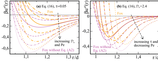
Figure B1. Closeups of the Fox results for the full effective potentials from equation (B.2) as in figure 3 (a) top right with additional data for \mathcal{D}_a=0.6 and \mathcal{D}_a=0.3 and (b) bottom right with additional data for \tau=0.0125 and \tau=0.00625 . The thinner lines correspond to the results without making the approximation in equation (B.2).
