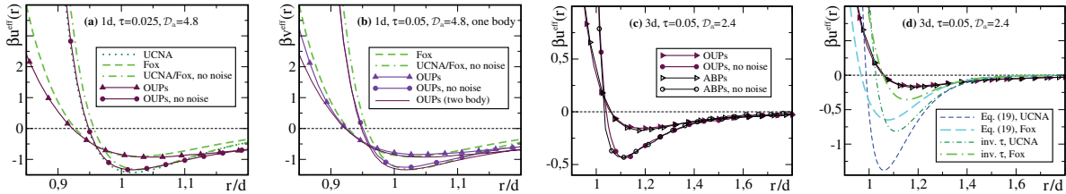
Figure 2. Effective potentials in a soft-repulsive system with and without thermal noise. (a) Comparison to simulations of active OUPS in \mathfrak{d}=1 with \mathcal{D}_a=4.8 and \tau=0.025 , as in figure 1(d), including the Fox approximation (dashed lines) and simulations without thermal noise (labeled with dots). In the latter case, UCNA and Fox are equivalent (dot-dashed line). (b) As figure 2(a), but for a single active particle in an external potential \beta\nu(r)=(r/d)^{-12} with \tau=0.05 chosen such that the theory predicts the same curves as for two particles with \tau=0.025 (the two-body simulation results for \tau=0.025 from figure 2(a) are shown as thin solid lines for comparison). (c) Simulations of two ABPs (empty symbols) and OUPs for \tau=0.05 and \mathcal{D}_a=2.4 in \mathfrak{d}=3 dimensions. (d) As figure 2(c) (with noise) compared to the Laplacian approximation, equation (19), and the inverse- \tau approximation as labeled.
