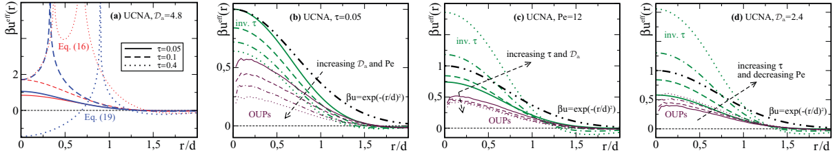
Figure 4. Effective potentials from the UCNA in three dimensions for Gaussian-core particles, \beta u(r) = \exp(-(r/d)^2) . (a) Comparison of the divergences in the full result from equation (16) and the Laplacian approximation, equation (19), for different persistence times \tau . (b)–(d) Inverse- \tau approximation and computer simulations for active OUPs for the same parameters as in rows 1–3 of figure 3, respectively. The bare potential is shown as the thick dot–dot–dashed line.
