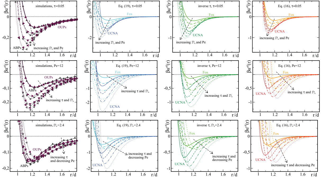
Figure 3. Effective potentials in three dimensions for soft-repulsive spheres, \beta u(r) = (r/d)^{-12} , obtained within the Fox (thick, brighter lines) and UCNA (thin, darker lines) and by numerical simulations of ABPs (empty triangles) and active OUPs (filled triangles). Columns from left to right: simulations; Laplacian approximation, equation (19); inverse- \tau approximation, equations (16) with (20); equation (16) only for r > r_{\text{div}} (see figure 1(a) for the full result). Rows from top to bottom: increasing the active diffusivity D_a at constant persistence time \tau = 0.05 ; increasing D_a and \tau at constant Péclet number Pe = \sqrt{3D_a/\tau} = 12 ; increasing \tau at constant D_a = 2.4 . The sequence from the solid to the dotted lines corresponds to increasing the respective parameter(s) D_a from D_a = 1.2 or \tau from \tau = 0.025 by a factor of two in each step (dashed lines are always for the same set of parameters).
