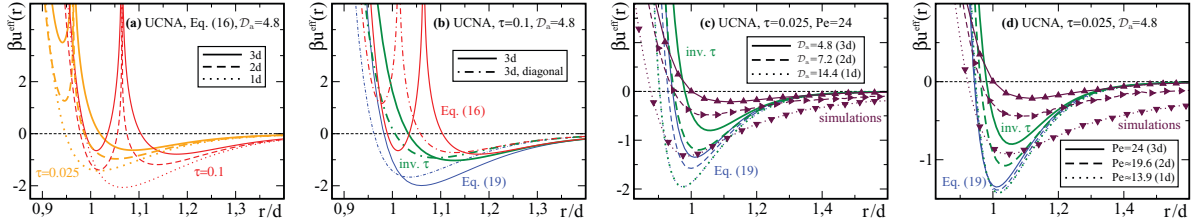
Figure 1. Effective potentials in the presence of thermal noise for a soft-repulsive \beta u(r) = (r/d)^{-12} from the UCNA in \mathfrak{d}=1 (dotted lines), \mathfrak{d}=2 (dashed lines) and \mathfrak{d}=3 (solid lines) dimensions. (a) Full result, equation (16), for the active diffusivity \mathcal{D}_a = 4.8 and persistence times \tau = 0.025 (thick, brighter lines) or \tau = 0.1 (thin, darker lines). (b) Comparison to the diagonal form (dot-dashed lines) in \mathfrak{d}=3 for \mathcal{D}_a = 4.8 and \tau = 0.1 . The thick lines correspond to the inverse- \tau approximation, equation (20) of equation (16), and the thin lines to the Laplacian approximation, equation (19). (c) Approximate results compared to simulations of active OUPS (lines with triangles) at \tau = 0.025 and a constant Peclet number Pe = \sqrt{\mathfrak{d}\mathcal{D}_a}/\tau = 24 , as \mathcal{D}_a increases with decreasing \mathfrak{d} . (d) Approximate results compared to simulations of active OUPS at \mathcal{D}_a = 4.8 and \tau = 0.025 .
