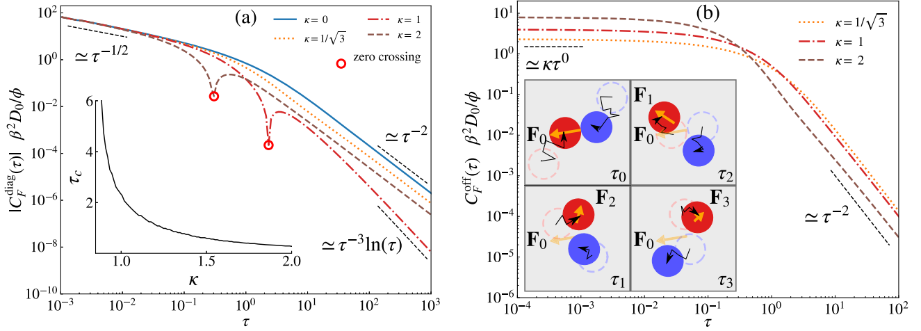
FIG. 1. Double-logarithmic plot of the diagonal and off-diagonal elements of the force autocorrelation tensor (FACT) of interacting hard disks as a function of reduced time \tau = t/\tau_0 , where \tau_0 = \sigma^2/(2D_0) . (a) The diagonal elements of the FACT C_F^{\text{diag}}(\tau) , corresponding to the force autocorrelation function (FACF), can turn negative. The FACF diverges in the limit \tau \rightarrow 0 as C_F^{\text{diag}}(\tau) \approx \tau^{-1/2} . At long times the FACF scales as C_F^{\text{diag}}(\tau) \approx \tau^{-2} . For \kappa = 1 we find an exceptional long-time behavior, where C_F^{\text{diag}}(\tau) \approx \tau^{-3} \ln(\tau) . The inset shows the zero-crossing time \tau_c of C_F^{\text{diag}}(\tau) as a function of \kappa , which in the main figure is marked by red circles. The onset of the anticorrelation corresponds to \kappa > \kappa_{\text{th}} \approx 0.88 . (b) The off-diagonal elements of the FACT C_F^{\text{off}}(\tau) are independent of time in the short-time limit C_F^{\text{off}}(\tau) \approx \kappa \tau^0 and are directly proportional to \kappa . In the long-time limit, they scale similarly to the diagonal elements as C_F^{\text{off}}(\tau) \approx \tau^{-2} for all \kappa . The inset in (b) shows typical configurations after a collision of particles, where the orientational change of the force (orange arrow) \mathbf{F}_i = \mathbf{F}(\tau_i) , i \in \{0, 1, 2, 3\} of the tagged particle (red) is indicated. The black arrows thereby indicate a possible trajectory from one frame to the next.
