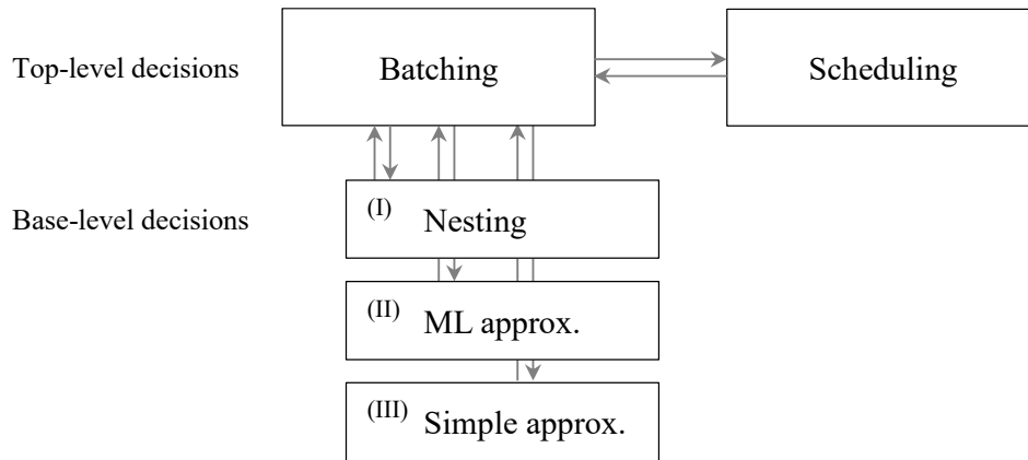
Figure 4: The BSP with approximation
