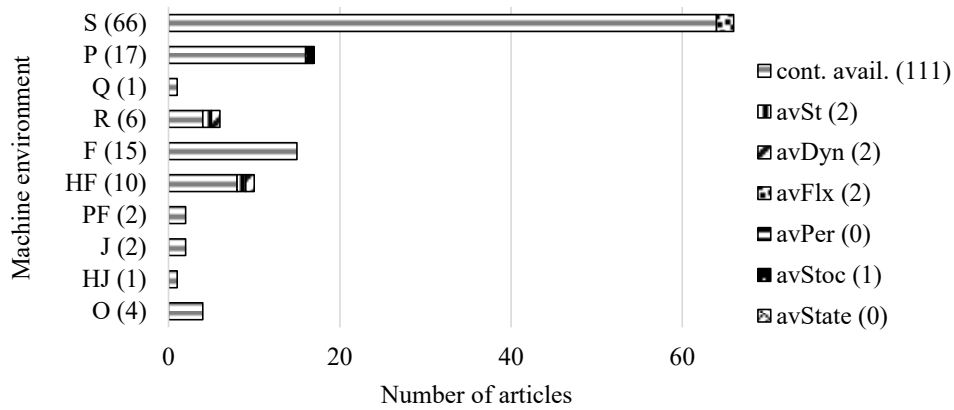
Figure 3: Machine environment (A1) and Machine availability (A3)
