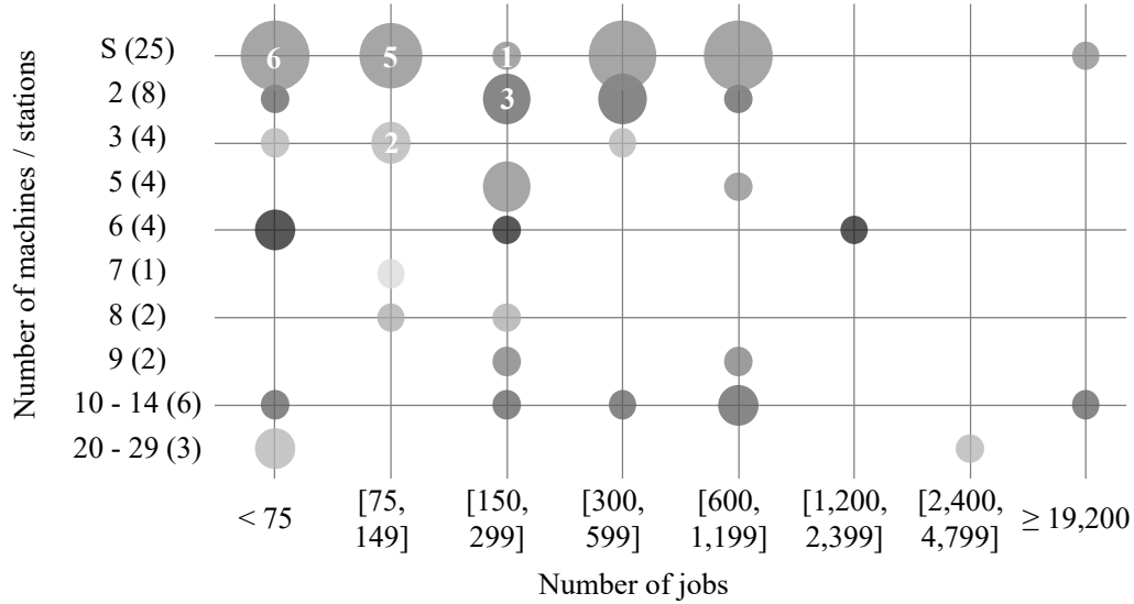
Figure 11: Number of articles in relation to the number of jobs and machines/stations (S representing single machine problems)
