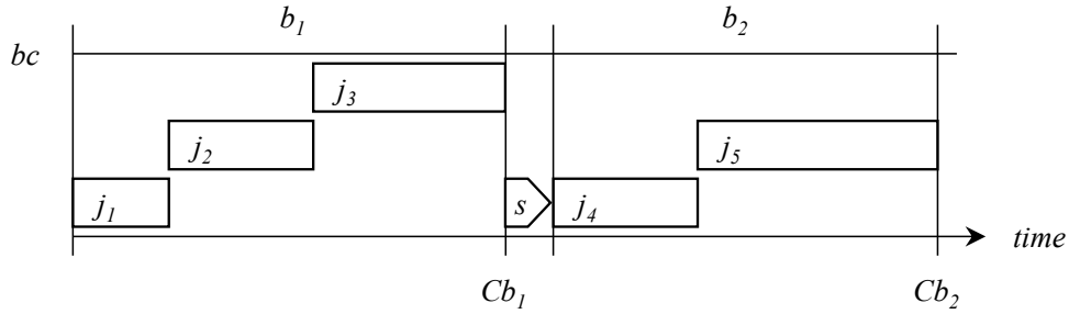
Figure 2: Batch scheduling with serial batching
