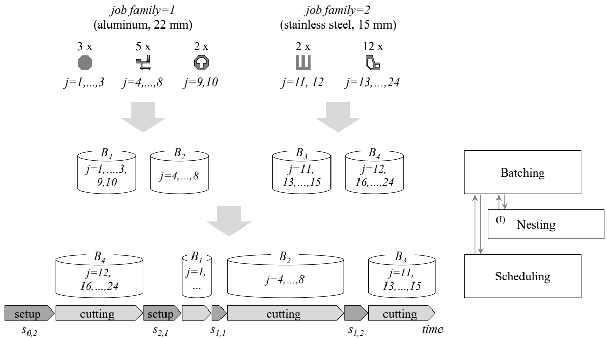
Figure 3: The serial-batch scheduling problem and its decisions
