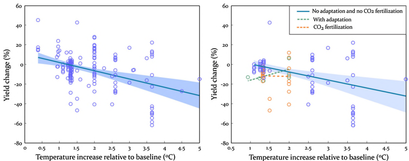
Fig. 6 Crop yield changes with temperature increase in the MENA region over all studies (left) and for studies that take the effects of adaptation measures (green line) and CO 2 fertilization (orange line) into account. The blue line in both panels indicates the best-fit line,
