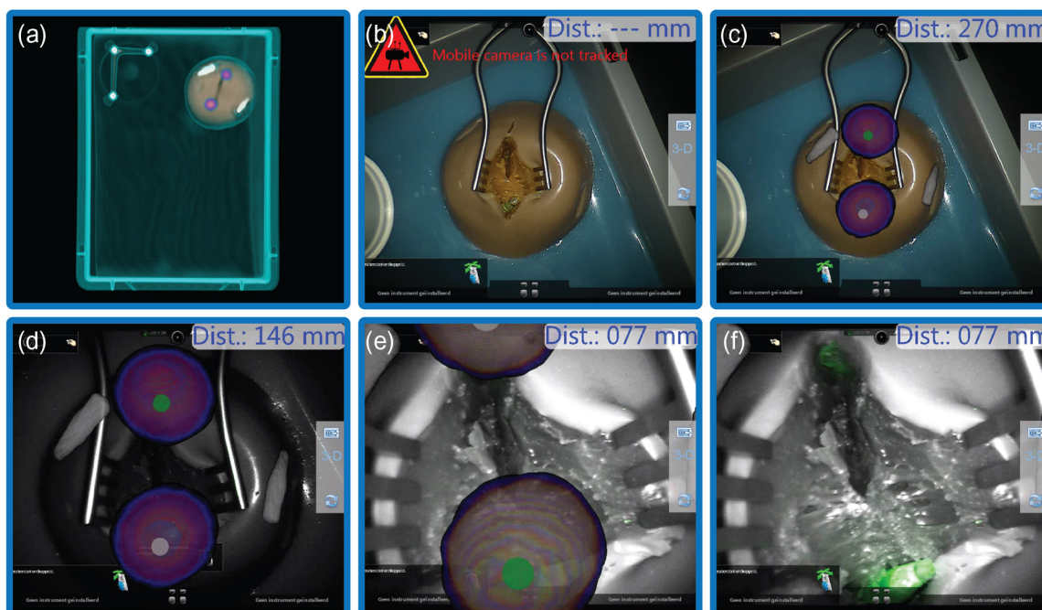
Fig. 2 Navigation of the fluorescence laparoscope based on preoperative SPECT/CT imaging and intraoperative fluorescence guidance as performed on the tissue-mimicking phantom setup. (a) Volume rendering of the fused SPECT/CT scan of the tissue-mimicking phantom setup. The SPECT hotspots are shown in purple/blue. (b–f) Augmented reality video feed from the perspective of the fluorescence laparoscope as seen on the navigation device, when navigating to the navigation targets. These targets are indicated as gray and green circles and are defined by the SPECT signal (displayed purple/blue). The distance shown is the distance from the tip of the camera to the selected (green) target. The CT overlay is shown in white/gray. (b) The phantom shown by white-light modus, without augmented SPECT/CT overlay. (An error states that the mobile camera is not tracked due to the LRT being just at the border of the tracking volume.) (c) White-light modus with augmented SPECT/CT overlay. (d and e) Fluorescence light modus with augmented SPECT/CT overlay. In this mode, the background video is shown in gray. (f) Fluorescence light modus without augmented SPECT/CT overlay. Fluorescence is displayed in green.
