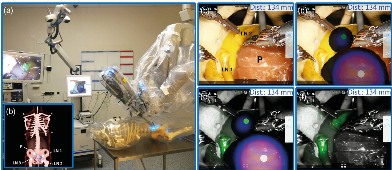
Fig. 4 Evaluation of the combined fluorescence navigation system based on preoperative SPECT/CT. (a) Operation room setup with the navigation system, fluorescence laparoscope, the surgical robot, and the torso phantom. On both the torso phantom and the fluorescence laparoscope, a reference target is attached. (b) Volume rendering of the fused SPECT/CT scan of the torso phantom setup. The SPECT hotspots are shown in pink/blue. The arrows indicate the prostate (P) and 3 lymph nodes (LN). (c–f) Augmented reality video feed from the perspective of the fluorescence laparoscope as seen on the navigation device when navigating to the navigation targets. These targets are indicated as gray and green circles and are defined by the SPECT signal (displayed purple/blue). The distance shown is the distance from the tip of the laparoscope to the selected (green) target. (c) White-light modus; letters indicating the specific lymph nodes (LN 1 and LN 2) and the prostate (P) in the anatomy of the phantom. (d) White-light modus with augmented SPECT overlay. (e) Fluorescence light modus with augmented SPECT overlay. (f) Fluorescence light modus without the augmented SPECT overlay. Lymph node LN 1 is located too close to the highly active prostate P (1 : 100 ratio in radioactivity) to resolve it as a separate navigation target by the used rendering.
