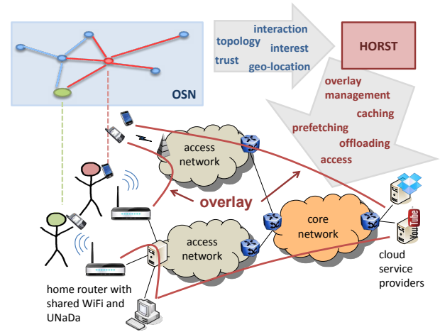
Fig. 1. Basic HORST functionality. HORST uses information from the OSN to provide end users access to shared WiFi access points based on their trust scores, to enable content prefetching and caching, and to control an efficient content delivery overlay.
