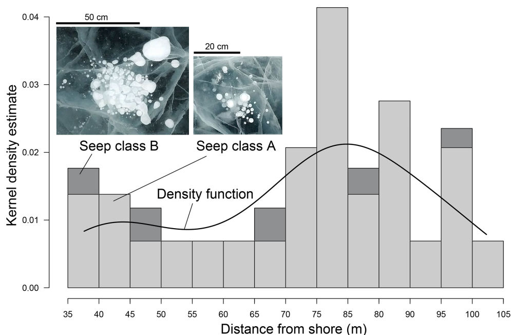
Figure 3. Distribution of \text{CH}_4 seeps of class A and B (Walter Anthony and Anthony, 2013) in Goltsovoye Lake (LK) perpendicular to the northwestern shore in a snow-cleared area of 70 \times 1.4 m. Bars represent the frequency of seeps A and B given as probability. The black line shows the kernel density function (Gaussian kernel performed on distances to shore; width is 34 data points).
