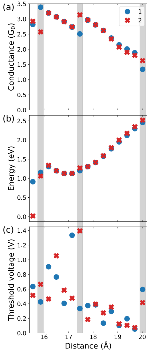
FIG. 2. (a) Conductance, (b) DFT energy, and (c) threshold voltage as a function of electrode separation distance d . Blue points visualize results obtained during an initial compression process. Red points are obtained through a mechanical cycle by separating the electrodes of the corresponding relaxed junction at the subsequent distance step d - \Delta by one distance step \Delta = 0.3 \text{ \AA} to reach the electrode separation d and relaxing the contact geometry again. The three gray bars indicate points of bistability in the conductance, as observed in panel (a).
