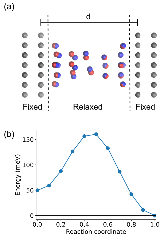
FIG. 4. Same as Fig. 3 but for d = 17.5 \text{ \AA} .
