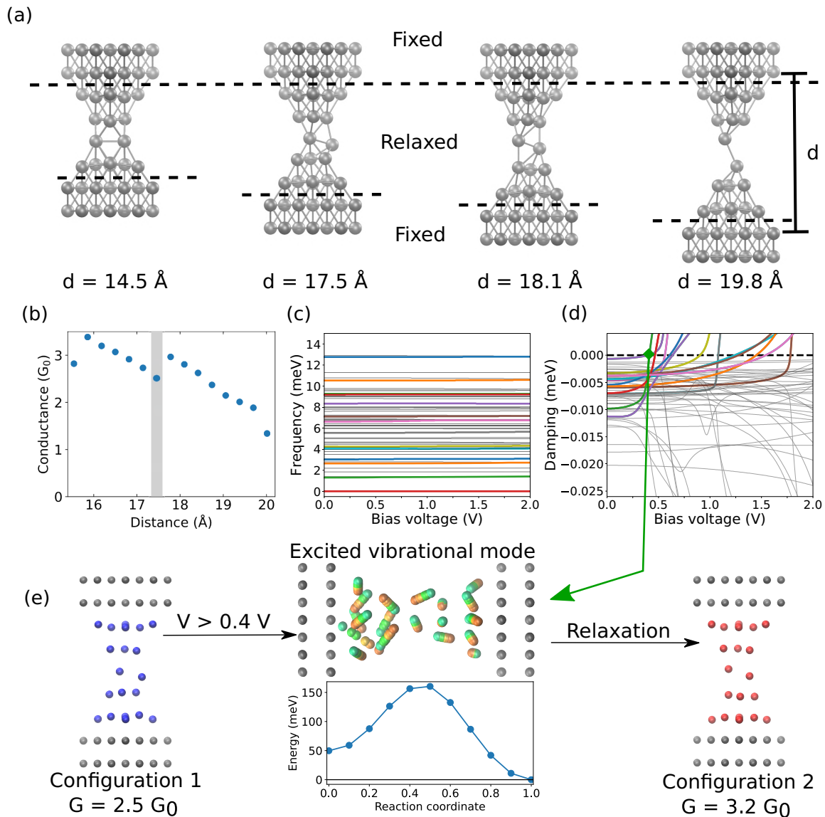
FIG. 1. Scheme of the simulation process for describing current-induced atomic rearrangements based on electron-vibration coupling. (a) Contact geometries at various electrode separations d . Fixed and relaxed atoms are separated by dashed lines. (b) Conductance as a function of the electrode separation d . The contact at d = 17.5 \text{ \AA} , which is studied further in panels (c)–(e), is marked in gray. (c) Vibrational frequencies as a function of the applied bias voltage for the contact at d = 17.5 \text{ \AA} . (d) Damping of the vibrations as a function of the bias voltage V for the contact at d = 17.5 \text{ \AA} . (e) Starting configuration 1 of the atomic contact (left, blue) at d = 17.5 \text{ \AA} ; displacement of its atoms by the mode with the lowest threshold voltage (middle), requiring V > 0.4 \text{ V} to become undamped. Contact configuration 2 (right, red) after a corresponding relaxation, i.e., energy optimization of atomic positions. The resulting junction configurations 1 and 2 exhibit different conductance of 2.5G_0 and 3.2G_0 , as indicated in the figure. The motion of atoms in the central relaxed junction part for one period of the unstable vibration is shown by snapshots in green and orange. The connection to the calculated bias-dependent damping in panel (d) is indicated by a green arrow. In the middle panel, the energy barrier between the two configurations is shown as a function of the reaction coordinate r .
