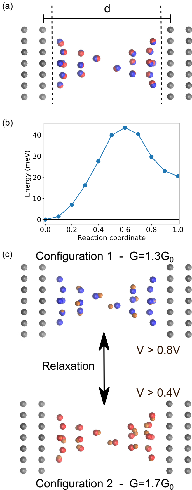
FIG. 5. (a) Contact configurations 1 (blue) and 2 (red) for d = 20 Å. (b) The configurations are separated by a reaction barrier of 20–40 meV, depending on the starting point. (c) The contact geometries in panel (a) realize a bistable switch between configuration 1
