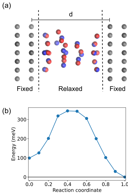
FIG. 3. (a) Contact configurations 1 (blue) and 2 (red) for the electrode separation d = 16 \text{ \AA} . (b) DFT energy as a function of the reaction coordinate r .
