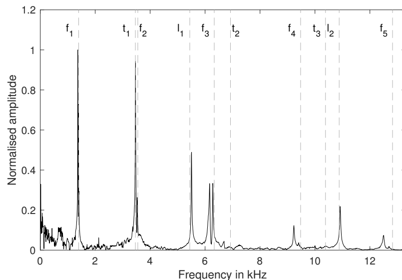
Figure 6. Spectral analysis of the impulse excitation data. The dotted lines mark natural frequencies based on FEM calculations, with Young's modulus and the shear modulus calculated analytically using f_1 and t_1 , respectively.
