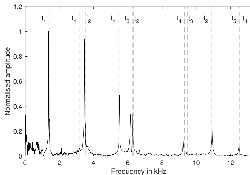
Figure 7. Spectral analysis of the impulse excitation data. The dotted lines mark natural frequencies based on FEM calculations. The Young’s and shear modulus of the FEM material model result from an error minimisation between the peaks in the spectrum and the calculated eigenfrequencies (<12 kHz).
