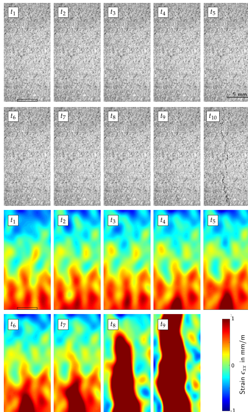
Figure 8. Strain calculation via digital image correlation for a 3-point-bending (3PB) experiment and 10 points in time ( t_1 – t_{10} ). Only the area under the punch is analysed. Starting at t_2 , the strain starts to localise until the fracture is complete at t_9 , which is still undetectable by the human eye. We added a scale to the plots
