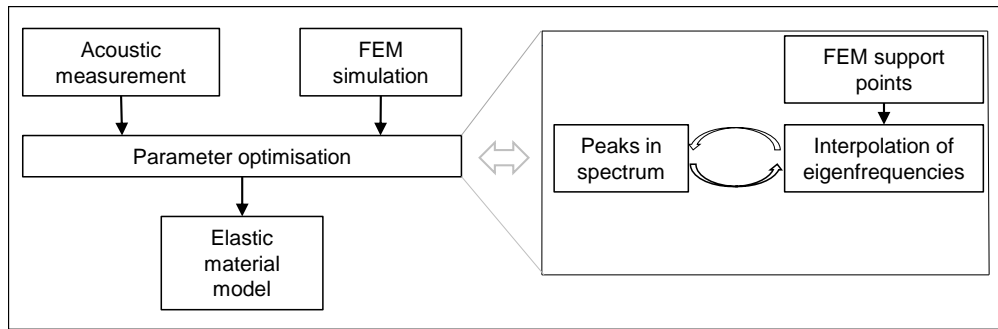
Figure 2. Algorithm for determining elastic parameters via impulse excitation technique and FEM simulation. The measured and calculated eigenfrequencies are compared and the Young’s modulus and Poisson ratio are optimised such, that the error between the measured and the calculated eigenfrequencies is minimal.
