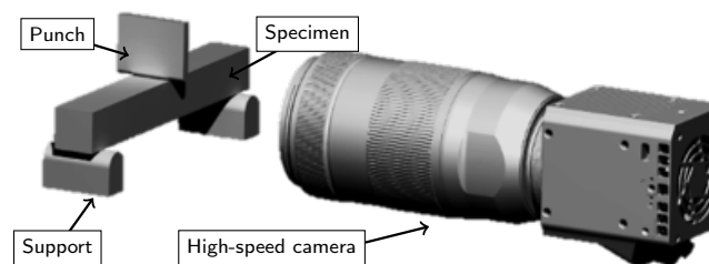
Figure 5. Test setup for a 3-point-bending experiment with high-speed imaging. The camera is oriented orthogonal to the specimen's surface.
