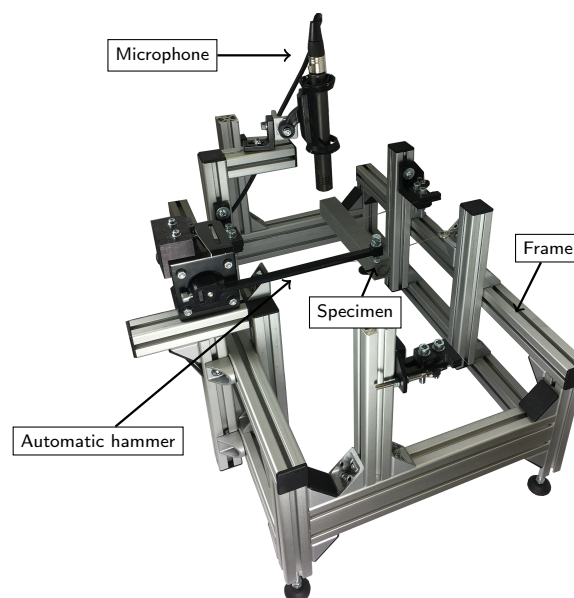
Figure 1. Test-bench for determining elastic properties via impulse excitation technique. The main components are a microphone, a specimen, an automatic hammer system and the frame of the test-bench.
