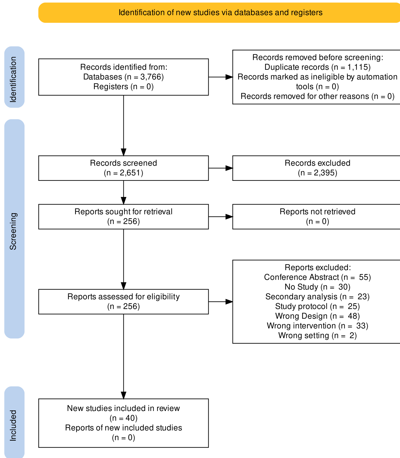
FIGURE 1 PRISMA flowchart.
