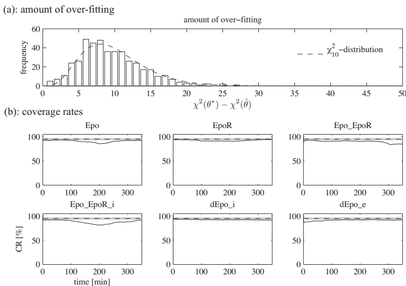
FIG. 6. The appropriateness of confidence intervals was assessed by a simulation study with 450 generated data sets. (a) Comparison of the amount of overfitting to the expected \chi^2_{df} distribution with df=10 . (b) The solid lines indicate the CRs for the time pointwise confidence bands on the model trajectories shown in Fig. 5(c). The dashed lines are the desired 95% level of confidence, while the gray shades are the expected coverage rates.
