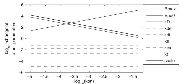
FIG. 4. Initial setup: the change of the other parameters along the profile likelihood \chi^2_{PL}(k_{on}) indicates functional relations between all five structural nonidentifiable parameter, indicated by the solid lines.
