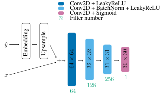
Figure 3: Architecture overview of the discriminator network.
