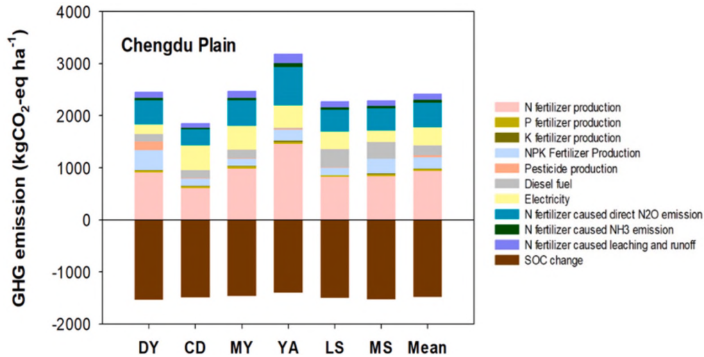
Fig. 5. GHG emissions and key components in different regions of the Chengdu Plain.
