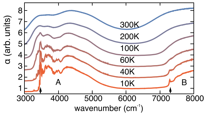
FIG. 4. Absorption spectra in \text{Fe}_2\text{Mo}_3\text{O}_8 for polarization configuration E^{\omega} \perp c & H^{\omega} \perp c at various temperatures crossing T_N = 60 K. Spectra are shifted for clarity with respect to the 10 K spectrum. Arrows mark the narrow onset excitations of the broad A and B bands.
