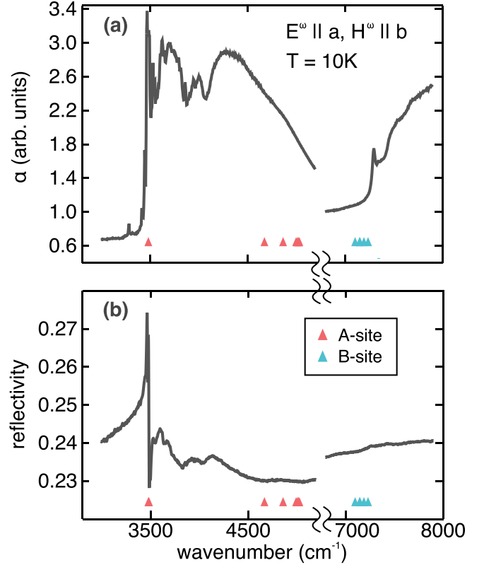
FIG. 8. Absorption and reflectivity spectrum in \text{Fe}_2\text{Mo}_3\text{O}_8 measured in the MIR/NIR frequency range with light polarization configuration E^\omega \perp c & H^\omega \perp c at 10 K and comparison with the calculated excitations as described in the text.
