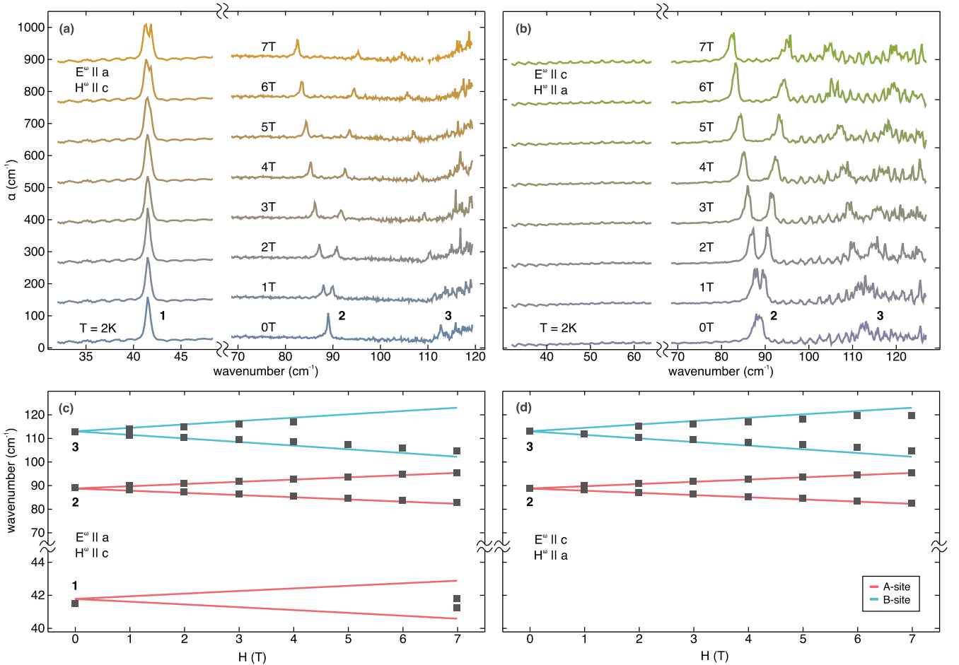
FIG. 3. Magnetic field dependence of the THz absorption spectra at 2 K with the external field \mathbf{H} \parallel c for polarization configurations (a) E^\omega \parallel a & H^\omega \parallel c and (b) E^\omega \parallel c & H^\omega \parallel a . Spectra in panels (a) and (b) are shifted with respect to the zero-field spectrum for clarity. Panels (c) and (d) show a comparison of the experimental eigenfrequencies (solid squares) for the spectra in (a) and (b), with the calculated field dependence (solid lines) as described in the text. Red lines refer to A-site related excitations, blue lines to a B-site related one.
