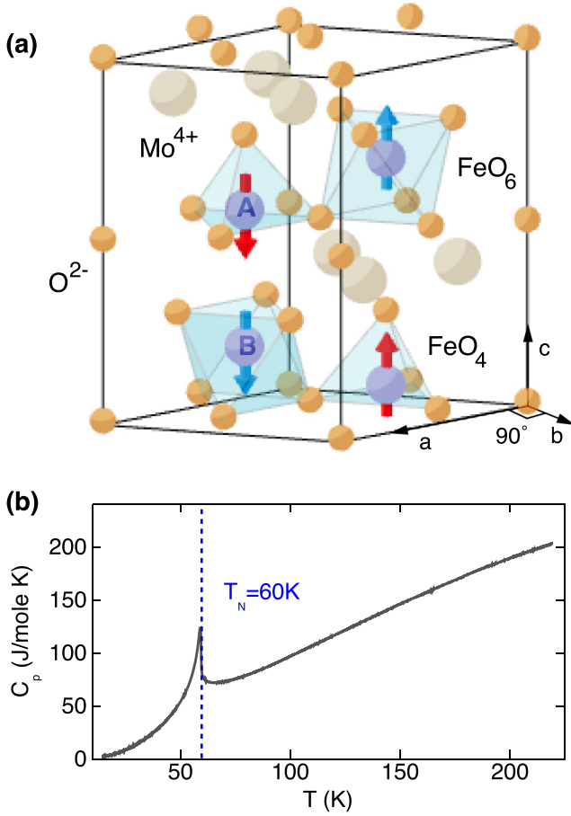
FIG. 1. (a) Unit cell of \text{Fe}_2\text{Mo}_3\text{O}_8 in the antiferromagnetic state with tetrahedral (a) and octahedral (b) sites shown in red and blue, respectively, and the polarization along the c axis. The depicted b axis is perpendicular to the hexagonal a axis. (b) Temperature dependence of the specific heat C_p showing the antiferromagnetic ordering at T_N = 60 K.
