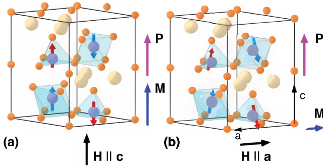
FIG. 6. Comparison of the two measurement configurations (a) with the external field applied along the polar antiferromagnetic c axis, where the Zeeman-like splitting occurs as shown in Fig. 3 and (b) with \mathbf{H} \parallel a , where nondirectional dichroism can occur.
