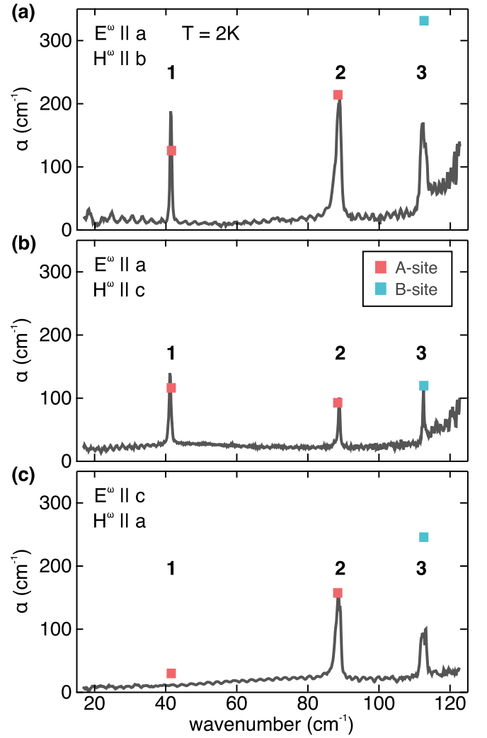
FIG. 2. Absorption coefficient in the THz range in \text{Fe}_2\text{Mo}_3\text{O}_8 for the three orthogonal light polarization configurations (a) E^\omega \parallel a & H^\omega \parallel b , (b) E^\omega \parallel a & H^\omega \parallel c , and (c) E^\omega \parallel c & H^\omega \parallel a at 2 K. The solid squares indicate the calculated absorption coefficient as described in the text, red refers to an A-site related excitation, blue to a B-site related one.
