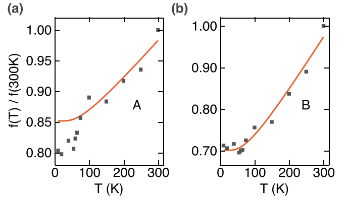
FIG. 5. Temperature dependence of the normalized integrated absorption strength f(T)/f(300\text{ K}) with a fit using f(T) = f_c + f_0 \coth(\hbar\omega/2k_B T) for (a) the A band and (b) the B band.
