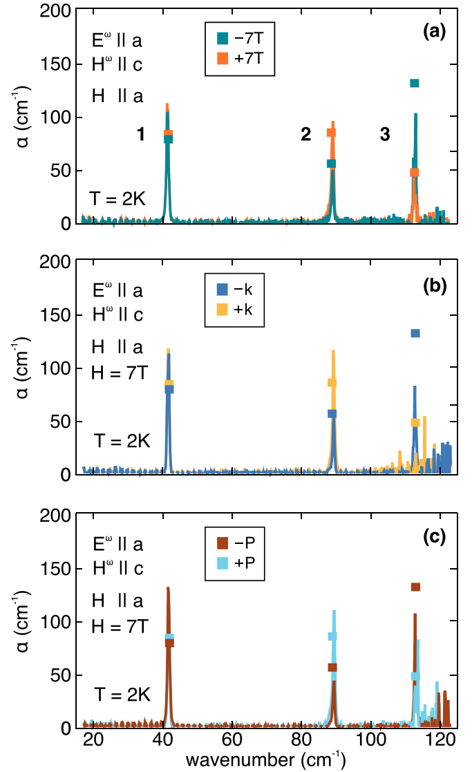
FIG. 7. Comparison of the absorption coefficient for polarization configuration E^\omega \parallel a & H^\omega \parallel c and an external magnetic field H = \pm 7 T applied along the crystallographic a axis. Symbols correspond to the calculated absorption coefficient at H = \pm 7 T as discussed in the text.
