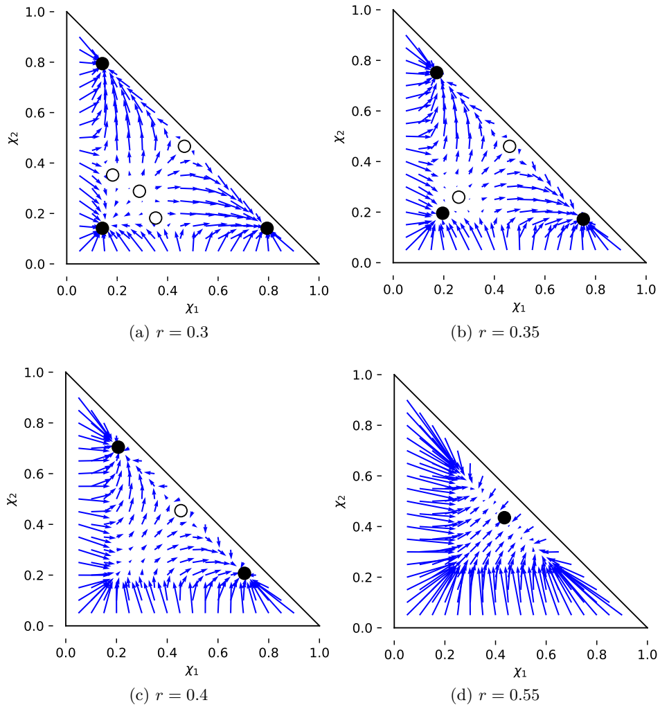
Figure 6.4: The field G (see (6.5)) with A = 3 , \beta = 2 , \alpha_1 = \alpha_2 = \alpha_3 = 1 and \gamma = (0.4, 0.4, 0.2) for various labor shares r . Stable fixed points are marked with • and unstable fixed points with o. Their exact position has been computed explicitly with Mathematica.
