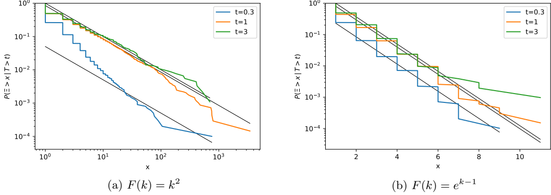
Figure 5.1: The empirical distribution of \Xi(t) conditioned on T > t for different F and t . The black lines show the predicted tail according to Theorem 5.1. 10,000 realizations of the process (5.2) were simulated each. In (a) 10 (resp. 3112, resp. 9088) have already exploded at time t = 0.3 (resp. t = 1 , resp. t = 3 ) and in (b) 30 (resp. 3424, resp. 8974). As the criterion for explosion, the simulation was stopped after 10^6 summands in (a) and 100 summands in (b).
