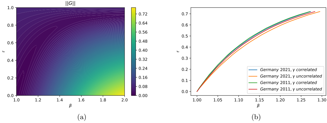
Figure 6.5: The left figure shows a contour plot of \|G(x_{ger})\| with a normalized sample x_{ger} from CDF_{ger} (6.9) for different values of r and \beta , where \gamma and x_{ger} are fully correlated. The right one shows the minimizing r - \beta -line for different years where \gamma and x_{ger} are fully correlated or uncorrelated.
