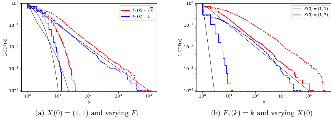
Figure 5.5: Empirical distribution of X_1(\infty) (full line) and N_{mon} (dotted line) for A = 2 , F_2(k) = k^2 and different F_1 and X(0) . The black lines show the tail decay predicted by Theorem 5.16 and Corollary E.6. Note that these predicted tails are only exact up to constants, i.e. up to a parallel shift in the plot. 10,000 simulations were executed each.
