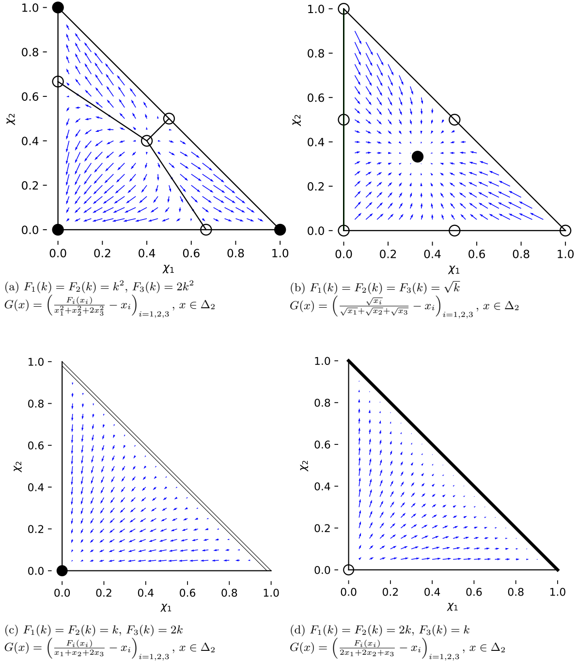
Figure 4.1: The vector field G for different feedback functions and A = 3 . Here \bullet marks the stable and \circ the unstable fixed points of the dynamics (4.2). In addition, Figure (a) shows the asymptotic attraction domains as derived in Example 3.16.
