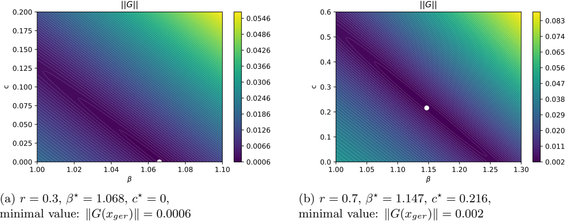
Figure 6.12: Contour-plot of \|G(x_{ger})\| for varying values of \beta and c , where r = 0.3 resp. r = 0.7 and x_{ger} are fixed. The white bullet marks the global minimum (\beta^*, c^*) . Note the different scales in both plots.
