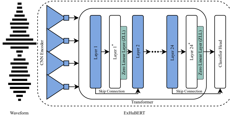
Figure 2: Outline of the proposed ExHuBERT architecture, including skip connections and zero linear layers. The CNN encoder and the weights of the layers colored in blue are frozen. The classifier head and the weights of the layers marked with an asterisk (*) will undergo fine-tuning during the evaluation process.
