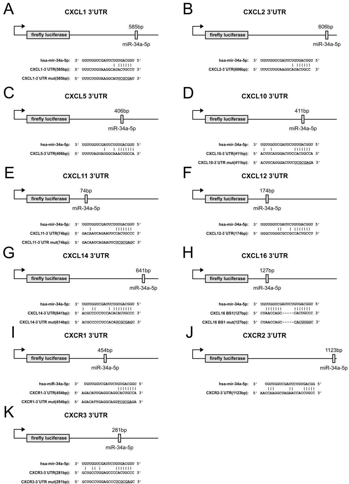
Figure 3 Schematic diagram of reporter gene plasmids. The position of the predicted miR-34a-5p binding sites in the respective 3'UTR reporter plasmids and their corresponding sequences as well as the sequences of the mutated binding sites (underlined) are shown. (A) CXCL1 -3'UTR reporter vector, (B) CXCL2 -3'UTR reporter vector, (C) CXCL5 -3'UTR reporter vector, (D) CXCL10 -3'UTR reporter vector, (E) CXCL11 -3'UTR reporter vector, (F) CXCL12 -3'UTR reporter vector, (G) CXCL14 -3'UTR reporter vector, (H) CXCL16 -3'UTR reporter vector, (I) CXCR1 -3'UTR reporter vector, (J) CXCR2 -3'UTR reporter vector, (K) CXCR3 -3'UTR reporter vector.
