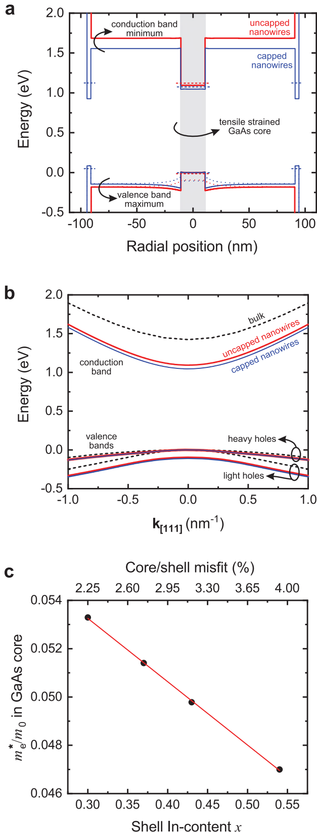
Fig. 2 Simulated electronic structure of the investigated GaAs/ \text{In}_{0.37}\text{Al}_{0.63}\text{As} core/shell (uncapped) and GaAs/ \text{In}_{0.43}\text{Al}_{0.57}\text{As} / \text{In}_{0.44}\text{Ga}_{0.56}\text{As} core/shell/capping-shell (capped) nanowires at 300 K using 8-band k - p theory. a Band-edge profile at the \Gamma -point of the Brillouin zone, along the [1\bar{1}0] crystallographic direction (from the middle of one side-facet, through the centre of the core at zero position, to the middle of the opposite side-facet). The valence bands for heavy and light holes are shown with continuous and dotted lines, respectively. The lowest confined energy levels in the core and the capping shell are indicated with horizontal dashed lines. b \Gamma -valley energy dispersion in the GaAs core, simulated along the [111] crystallographic orientation. One conduction and two valence bands (heavy and light holes) are shown. Results for unstrained bulk are also shown (black dashed lines) for comparison. The valence band maximum at \mathbf{k}_{[111]} = 0 has been set to zero energy. c Simulated dependence of the electron effective mass in the GaAs core on the In-content x of the \text{In}_x\text{Al}_{1-x}\text{As} shell (bottom x-axis) and the corresponding core/shell misfit (top x-axis). The data points are calculated values, which have been linearly fitted.
