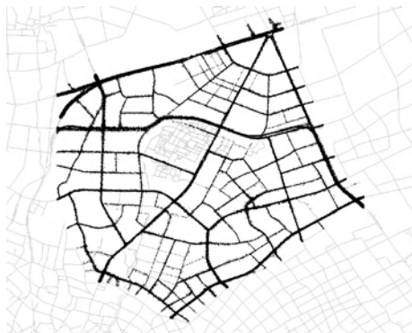
Figure 10. The GPS points in the test area.
