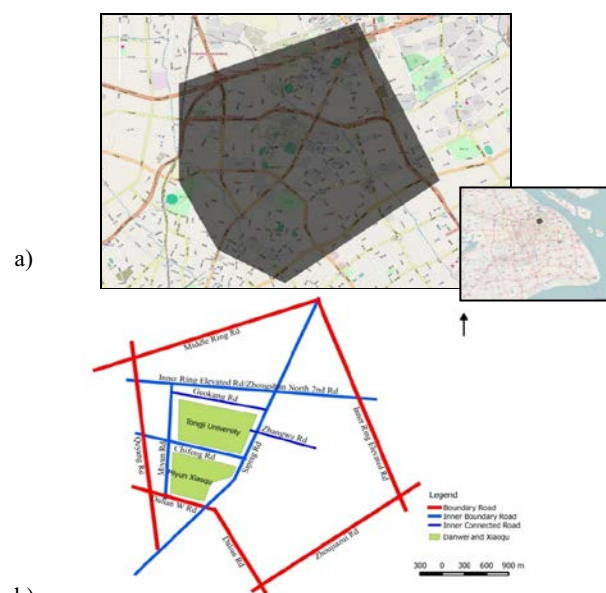
Figure 6 a) Study area in Shanghai, China. Study area is covered by a light grey shadow. Open Street Map (OSM) is used as base map, b) Sketch map for study area
