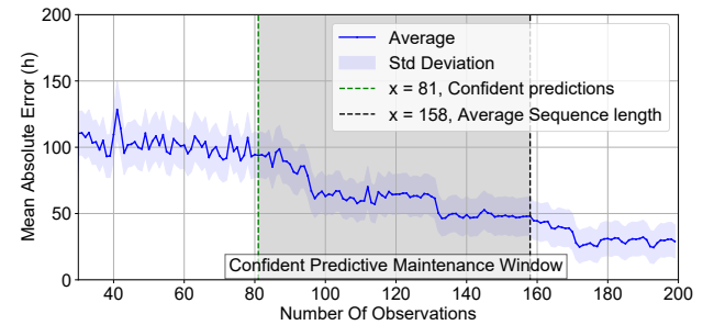
Figure 6: Evolution of the MAE in function of the number of observations for the best performing model.
