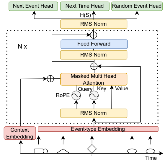
Figure 3: CarFormer architecture
