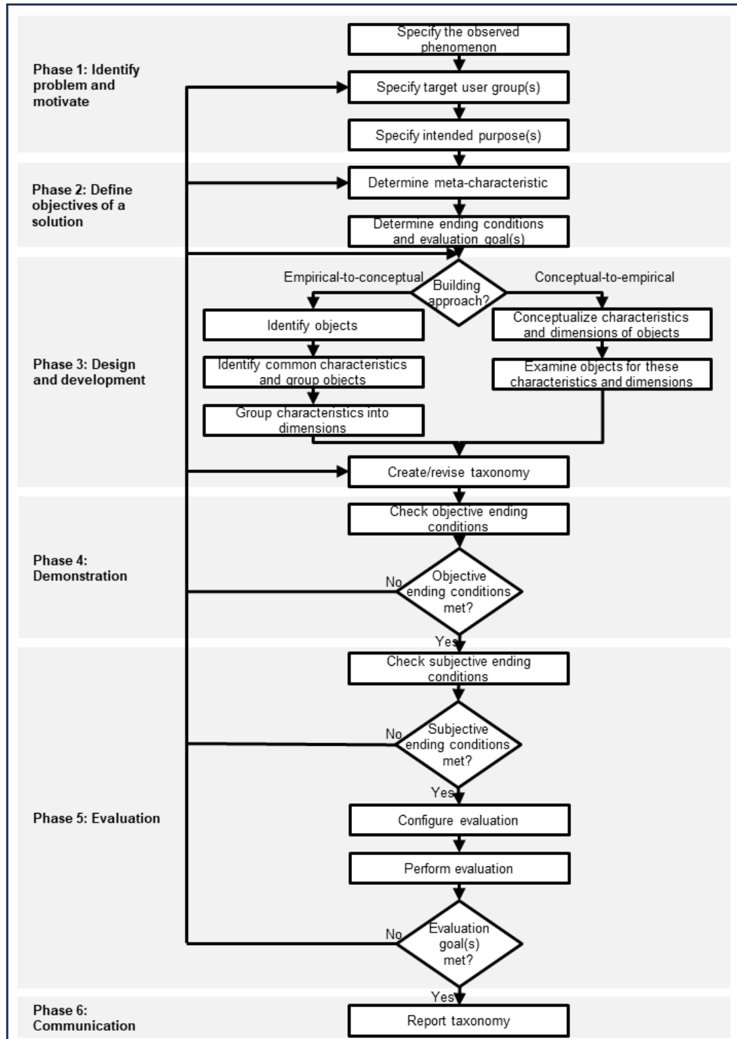
Figure 31: Steps Involved in Smart Urban Agriculture Taxonomy Design and Evaluation Process
