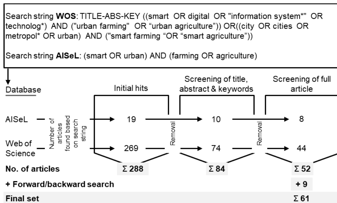
Figure 32: Search Protocol for Smart Urban Agriculture
