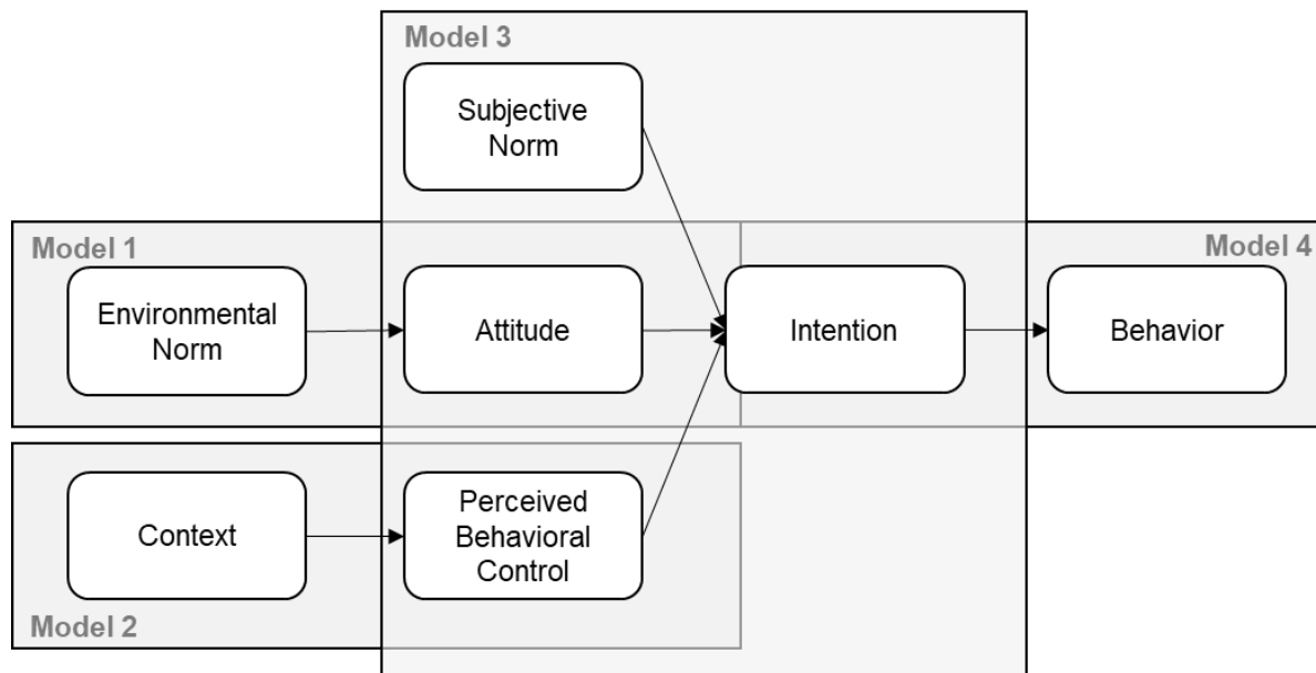
Figure 19: Regression Models
