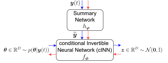
Fig. 1. BayesFlow architecture. \varphi, \phi denote the network parameters of the summary network h and the cINN f , respectively. The blue arrows represent the forward training process; the red arrows represent the inverse inference process. In the inverse process, only the cINN part is inverted, and the summary network part remains the same as that in the forward process.
