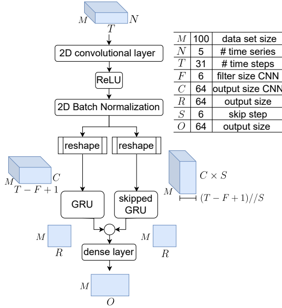
Fig. 2. LSTNet architecture.
