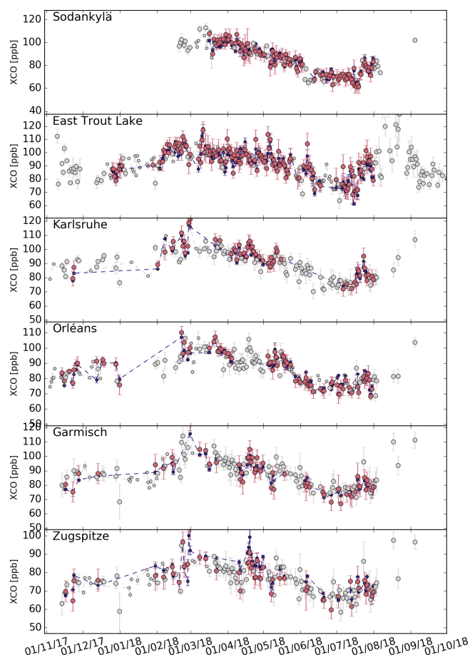
Figure 1. Daily mean of dry air column mixing ratios (XCO) measured by TROPOMI (pink) and various TCCON stations (blue) under clear-sky and cloudy atmospheric conditions. A colocation radius of 50 km is used. The standard deviation of individual retrievals within a day is shown as an error bar. The retrieval deployed the spectroscopic database HITRAN 2016 for all trace gases. Measurements of both datasets that could not be paired are marked as gray dots (big = TROPOMI, small = TCCON) and are not used in this study.
