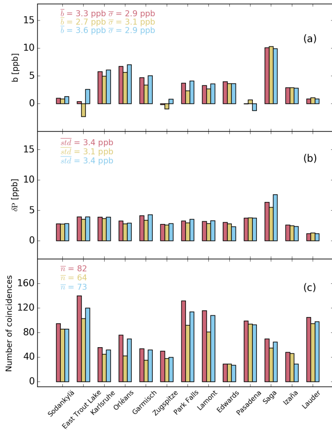
Figure 5. The same as Fig. 3 but comparing TCCON measurements with CAMS-IFS CO model data, which are colocated with the TROPOMI observations of Fig. 3. To this end, we interpolated the CAMS-IFS model temporally and spatially to TROPOMI measurements and also applied the averaging kernels of TROPOMI on the vertical profiles of the model. In this model comparison a spectral fit quality (rms) plot is not needed and is therefore replaced by the number of coincidences.
