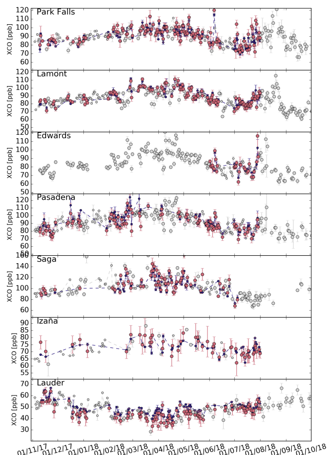
Figure 2. The same as Fig. 1 but for different TCCON stations.
