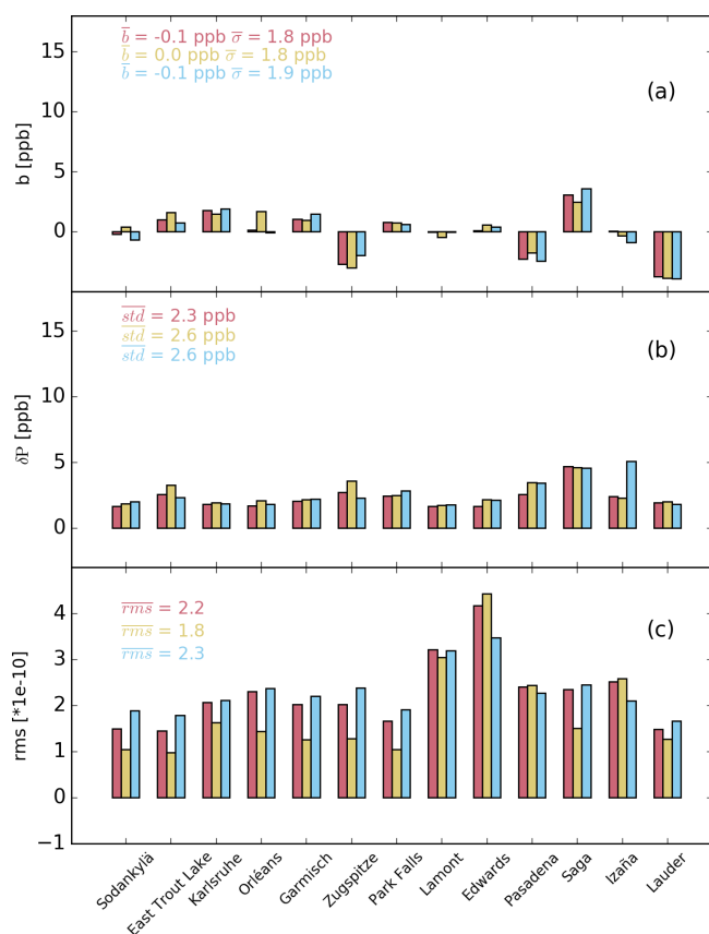
Figure 3. (a) Median bias b_j (TROPOMI-TCCON) for different TCCON sites between colocated daily mean XCO values of TROPOMI and TCCON (see blue and pink dots in Figs. 1 and 2) The global mean bias \bar{b} and the corresponding standard deviation \bar{\sigma} as defined in Eqs. (2) and (3), (b) the scatter \delta P_j of the biases as defined in Eq. (1) with its global mean \bar{\delta P} , and (c) the median root-mean-square (rms) of the spectral fit residuals of the individual retrievals per station and its global mean \bar{rms} in \text{mol s}^{-1} \text{m}^{-2} \text{nm}^{-1} \text{sr}^{-1} . The figure shows TROPOMI retrievals under clear-sky conditions (yellow), cloudy-sky conditions (blue) and the combination of both (pink). No destriping is applied to the TROPOMI data. The retrieval deploys the spectroscopic database HITRAN 2016 for all absorbers.
