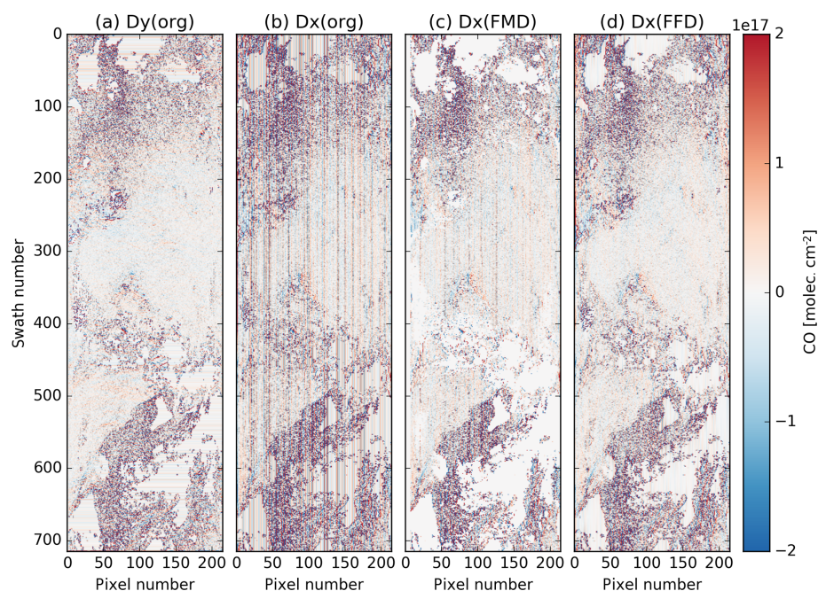
Figure 9. CO retrievals of one TROPOMI orbit on 28 July 2018 (partly shown). From left to right – (a) derivative Dy(d) along-track direction of the original data, (b) Dx(d) derivative in the cross-track direction of the original data, (c) Dx(d_{ds}) after FMD destriping and (d) is the same as (c) but after FFD destriping.
