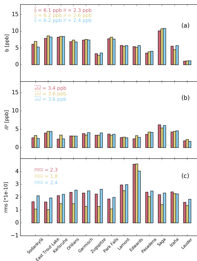
Figure 4. The same as Fig. 3 but deploying the spectroscopic database used in the operational TROPOMI CO processing (HITRAN 2008 with H 2 O updates).
