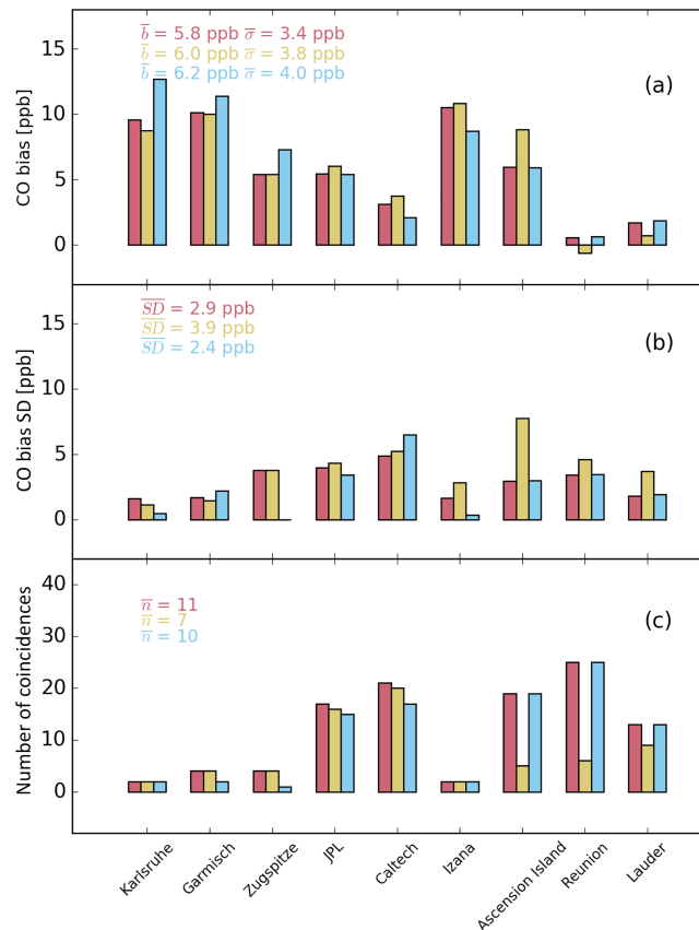
Figure 5. Mean bias (TROPOMI – FTS) between co-located daily mean XCO values (see Figs. 3, 4) of TROPOMI and TCCON (a), the standard deviation of the bias (b), and the number of coincident daily mean pairs (c). \bar{b} is the global mean bias (average of all station biases) and \bar{\sigma} its standard deviation. \bar{SD} is the average of all standard deviations and \bar{n} the average number of coincident pairs. TROPOMI retrievals under clear sky (yellow), cloudy sky (blue) and the combination of both (pink) are distinguished. No de-stripping was applied on the TROPOMI data.
