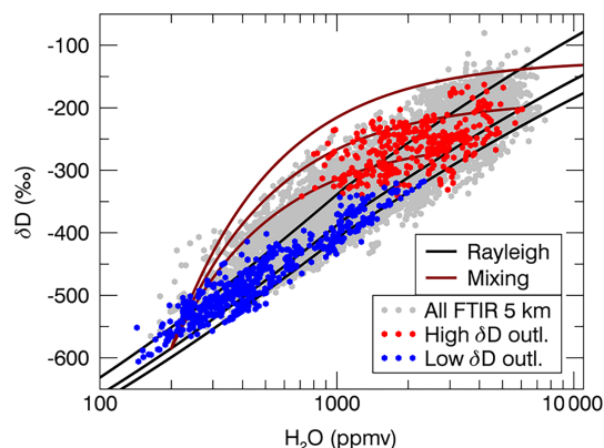
Figure 5. Free-tropospheric measurements of \{H_2O, \delta D\} pairs above Zugspitze (5 km a.s.l.) for all 2005–2015 data and for high and low \delta D outliers as determined from the deseasonalized column-based \delta D time series. For comparison, simulated Rayleigh processes (initial evaporation at T = 15^\circ\text{C} ; RH = 80\% ; \delta D values of -60 , -130 , and -160\text{‰} ) as well as mixing processes of upper-tropospheric air ( \text{VMR}_{H_2O} = 200 ppmv, \delta D = -585\text{‰} ) with three lower-middle-tropospheric air masses (i) \text{VMR}_{H_2O} = 13\,500 ppmv, \delta D = -130\text{‰} ; (ii) \text{VMR}_{H_2O} = 6100 ppmv, \delta D = -200\text{‰} ; (iii) \text{VMR}_{H_2O} = 3000 ppmv, \delta D = -270\text{‰} ) are shown.
