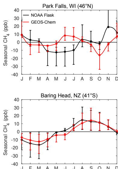
Figure 8. NOAA surface flask (black) and GEOS-Chem surface level (red) seasonality of \text{CH}_4 DMFs over 2005–2011 at Park Falls, WI, USA and Baring Head, NZ. Lower and upper bounds denote the 25th and 75th percentiles, respectively, of detrended data for each month.
