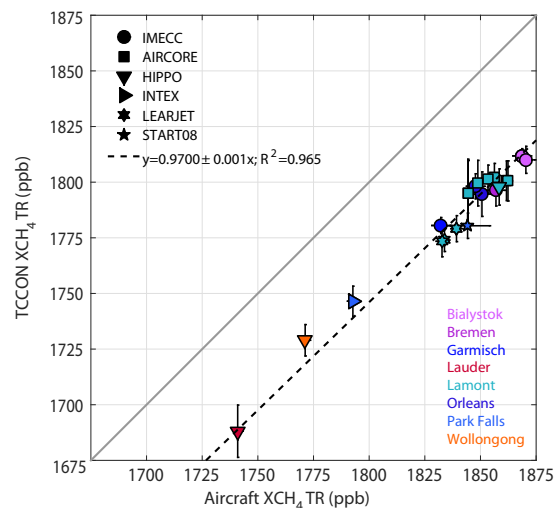
Figure A2. Calibration curve of TCCON X_{\text{CH}_4}^t (cf. Wunch et al., 2015, their Fig. 8). Site colors are as in Fig. 1. Aircraft campaigns are described in Table 6 of Wunch et al. (2015).
