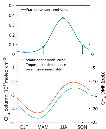
Figure 9. Top: Seasonally averaged fraction of model emissions from seasonally varying sources, north of 40^{\circ} N. Bottom: Seasonally averaged normalized model stratospheric column error (teal) and the difference between base and aseasonal simulation tropospheric columns (orange) at Park Falls.
