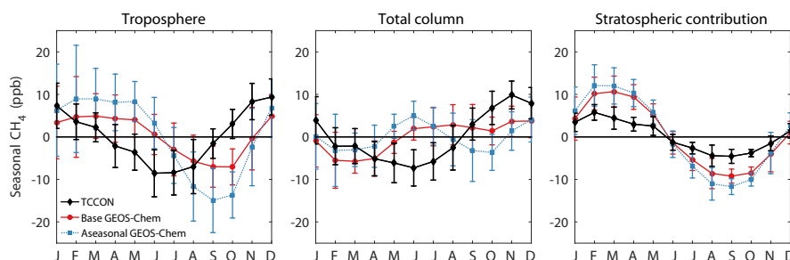
Figure 7. Detrended seasonality of TCCON (black diamonds), GEOS-Chem base (red circles), and GEOS-Chem aseasonal (blue squares) \text{CH}_4 column-averaged DMFs, averaged across Northern Hemisphere sites, excluding Saga, which has less than one year of measurements prior to 2012. Error bars denote the 1\sigma standard deviation across sites.
