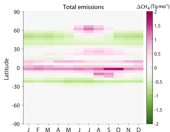
Figure B1. Monthly averages of the difference in total CH 4 emissions between the base and aseasoneal GEOS-Chem simulations, summed over each zonal band, in Tg mo −1 .
