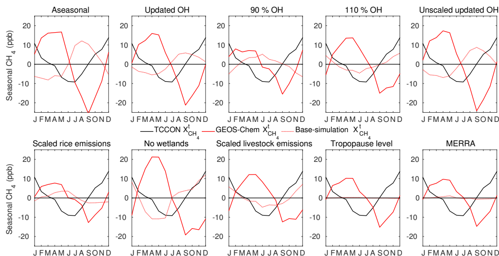
Figure B3. Seasonality of tropospheric methane ( X_{\text{CH}_4}^t ) at Park Falls for TCCON (black solid line), GEOS-Chem (red solid line), and the difference from the base simulation (dotted red line) for each of the sensitivity experiments, in ppb.
