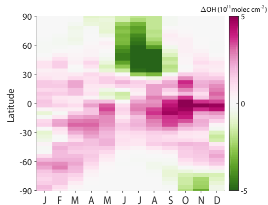
Figure B2. Zonal averages of the difference in total column OH (molecules cm −2 ) between the base and updated monthly OH fields.
