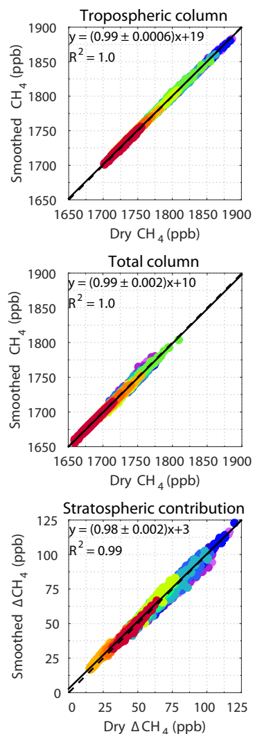
Figure B4. GEOS-Chem smoothed vs. dry integrated \text{CH}_4 DMFs for base simulation tropospheric columns, total columns, and stratospheric contribution. Site colors are as in Fig. 1. Dashed lines mark the one-to-one lines.
