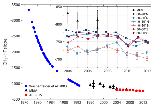
Figure A1. Long-term \text{CH}_4 -HF slopes from Washenfelter et al. (2003), MkIV, and updated ACE-FTS measurements. Inset: Time series of zonal pressure-weighted ACE-FTS slopes ( \beta ) used to calculate \hat{X}_{\text{CH}_4}^t , with error bars denoting the 2\sigma standard error. Zonal slopes are offset each year for visual clarity.
