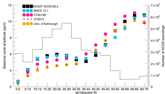
Figure 7. Latitudinal dependence of the seasonal cycle amplitude for bias-corrected ACOS B3.5 soundings and for three models re-sampled at the satellite soundings. For CarbonTracker, we show both CT2013 and CT2013B results, their difference being a major correction in the TM5 transport model. The left vertical axis shows the seasonal cycle amplitude in ppm, while the right vertical axis indicates the number of soundings that fall within each 5^\circ latitude band (black line).
