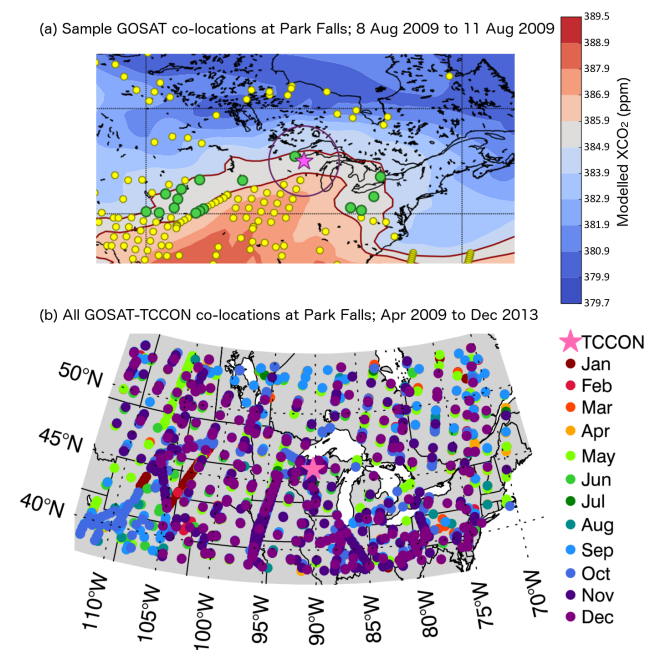
Figure 2. (a) An example of the GOSAT-TCCON co-locations using the NOAA/Basu technique (Guerlet et al., 2013a) at Park Falls TCCON station (Wisconsin, USA). All GOSAT/ACOS soundings from 8 to 11 August 2009 are shown with filled circles. The dynamical criterion based on the modelled XCO_2 fields and a 0.5 ppm tolerance from the value at the TCCON location limits the number of co-located satellite soundings (green circles). The soundings marked with yellow symbols did not pass the co-location criteria. (b) All co-located GOSAT/ACOS soundings from April 2009 to December 2013 at the Park Falls TCCON, coloured according to the month of observation.
