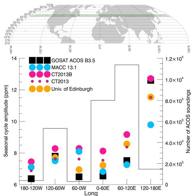
Figure 8. Longitudinal dependence of the seasonal cycle amplitude within the latitude band 45\text{--}50^\circ N. The left vertical axis shows the seasonal cycle amplitude in ppm, while the right vertical axis indicates the number of soundings that fall within each 60^\circ longitude bin. This latitude zone is highlighted in the world map where also the locations of the continents can be seen.
