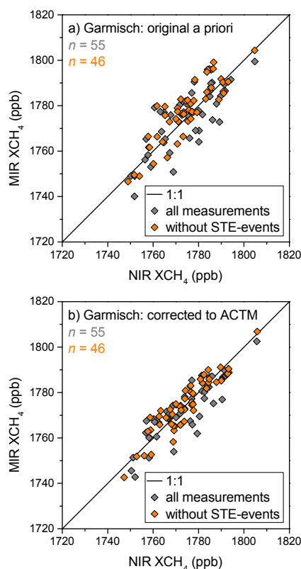
Figure 9. Scatter plot of MIR and NIR monthly means for Garmisch \text{XCH}_4 obtained from all FTIR measurements (black diamonds) and FTIR measurements which are not affected by STE events (red diamonds), respectively. (a) MIR and NIR \text{XCH}_4 retrieved with their original retrieval a priori profiles and (b) a posteriori corrected to common ACTM profiles. Note: the data set is not identical to that in Sect. 3 because STE trajectories are not available for the complete time series.
