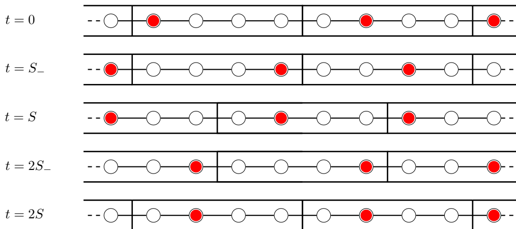
Figure 1: Illustration of the censoring scheme used in the proof of Proposition 5.2 with U = 2 . During each period [iS, (i + 1)S) for i \in \mathbb{N}_0 , the particles shown in red are only allowed to move within their assigned boxes.
