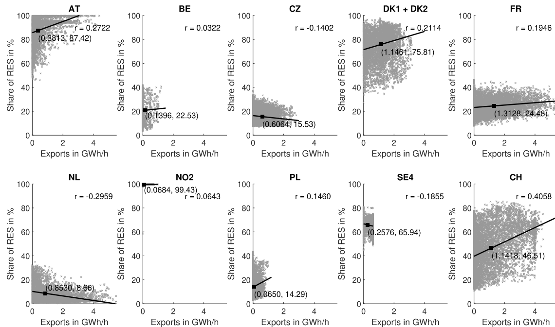
Fig. 4. Cumulative commercial exports of its neighboring countries to Germany and the corresponding share of RES in the corresponding country Own illustration, data from Refs. [51,53].
