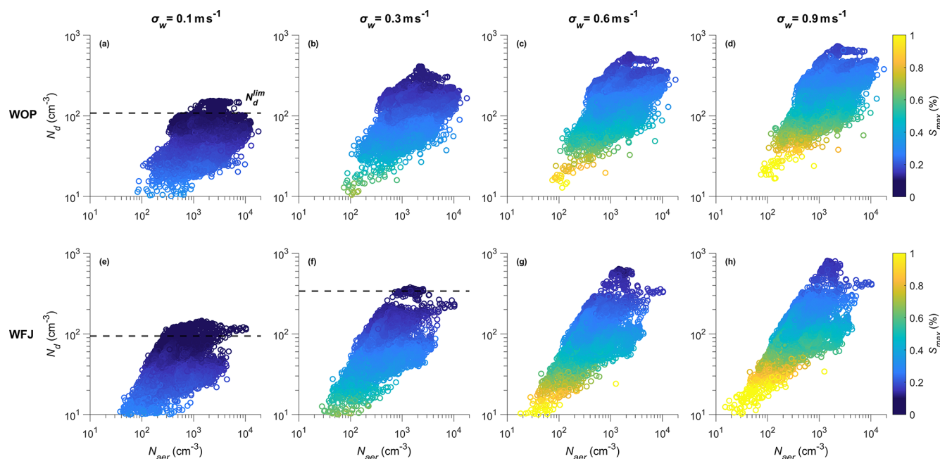
Figure 8. In situ N_d ( \text{cm}^{-3} ) vs. N_{aer} ( \text{cm}^{-3} ) for updraft velocities of \sigma_w = 0.1 \text{ m s}^{-1} in panels (a) and (e), 0.3 \text{ m s}^{-1} in panels (b) and (f), 0.6 \text{ m s}^{-1} in panels (c) and (g), and 0.9 \text{ m s}^{-1} in panels (d) and (h) during the period of interest at WOP (top panels) and WFJ (bottom panels). Data are colored by S_{max} (%).
