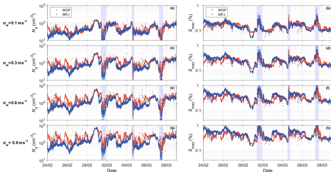
Figure 7. Calculated time series of N_d ( \text{cm}^{-3} ) (left panels) and S_{\text{max}} (%) (right panels) for updraft velocities of \sigma_w = 0.1 \text{ m s}^{-1} in panels (a) and (b), 0.3 \text{ m s}^{-1} in panels (c) and (d), 0.6 \text{ m s}^{-1} in panels (e) and (f), and 0.9 \text{ m s}^{-1} in panels (g) and (h) during the period of interest at WOP (orange dots) and WFJ (blue dots). The blue shaded areas represent the intense precipitating periods shown in Fig. 2.
