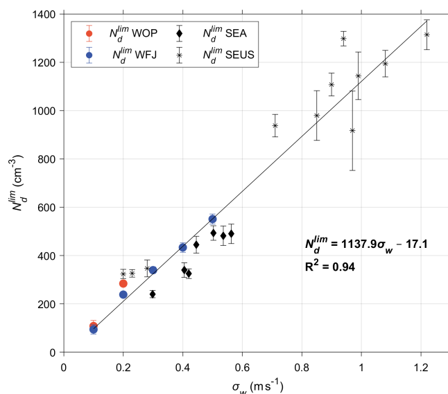
Figure 9. N_d^{lim} ( \text{cm}^{-3} ) against \sigma_w ( \text{m s}^{-1} ) calculated when velocity-limited conditions are met at WOP (orange circles) and WFJ (blue circles) throughout the period of interest. Superimposed are the corresponding values calculated for clouds forming over the SEA Ocean (rhombuses) and over the SEUS (asterisks).
