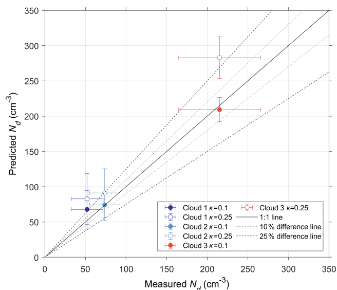
Figure 6. Comparison between average predicted N_d ( \text{cm}^{-3} ) with the droplet activation parameterization and observed N_d ( \text{cm}^{-3} ) during the three cloud events on 7 March (blue and cyan circles) and 8 March (orange circles) 2019. For all three cloud events, droplet closure is performed assuming a \kappa parameter of 0.1 (filled circles) and 0.25 (empty circles). The error bars represent the standard deviation of N_d during each cloud event.
