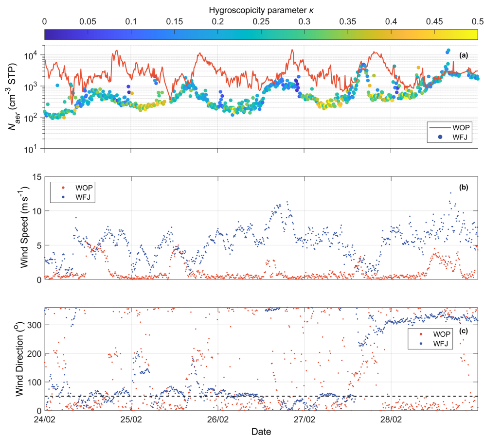
Figure 1. (a) N_{\text{aer}} under standard temperature and pressure conditions ( \text{cm}^{-3} STP) at WOP (orange line) and at WFJ (circles colored by \kappa ), (b) wind speed ( \text{m s}^{-1} ), and (c) wind direction (in degrees) obtained from the MeteoSwiss observation stations at WFJ (blue dots) and Davos (orange dots) between 24 and 28 February 2019. The black dashed line indicates the relative direction of WOP to WFJ. Each day is referenced to 00:00 UTC.
