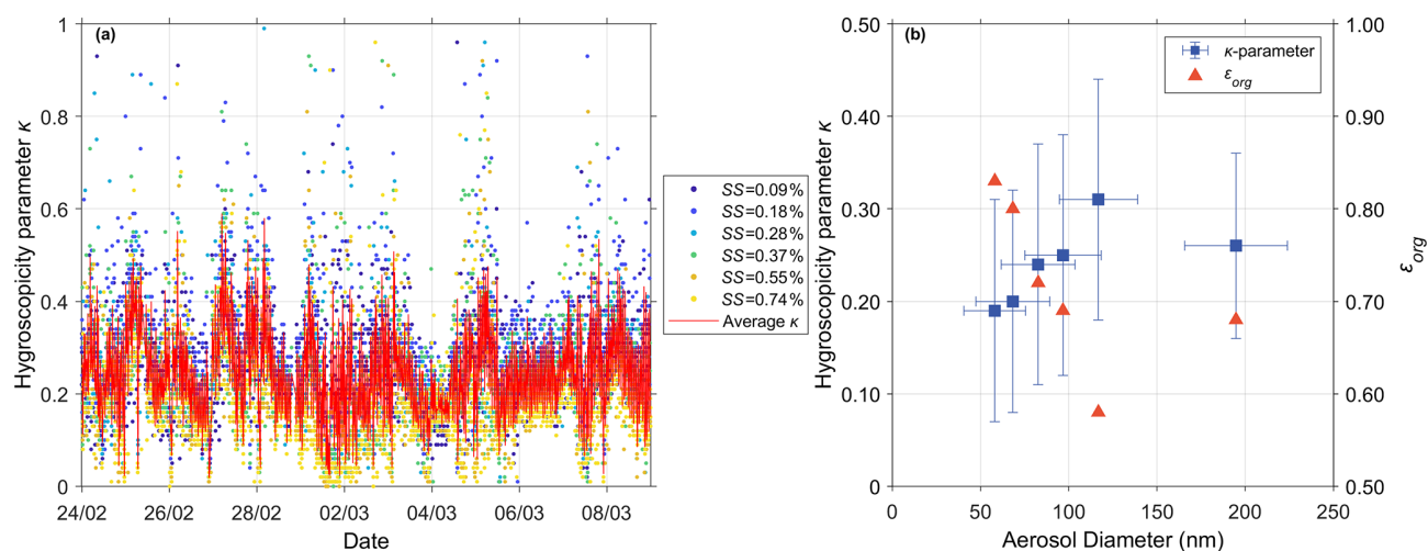
Figure 4. (a) Time series of the hygroscopicity parameter \kappa at WFJ at different levels of SS (0.09 %–0.74 %) throughout the period of interest. The red solid line indicates the hourly averaged \kappa time series over a complete SS cycle. (b) Size-resolved aerosol hygroscopicity (blue squares) and the respective \epsilon_{org} (orange triangles) calculated for the WFJ site.
