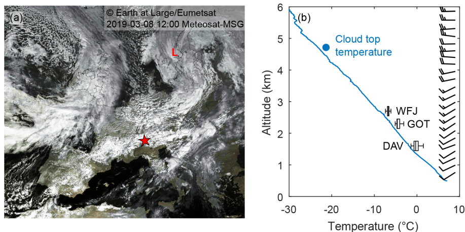
Figure 2. Overview of the synoptic weather situation on 8 March 2019, showing a satellite picture taken over Europe at 12:00 UTC (a, EU-METSAT) and the vertical temperature profile measured by a radiosonde (12:00 UTC) launched from Payerne (b, MeteoSwiss). The boxplots in (b) indicate the temperature measured at the weather stations of Davos (DAV, 1600 m), Gotschnagrat (GOT, 2300 m) and Weissfluhjoch (WFJ, 2700 m) during the passage of the cloud system. The blue dot indicates the cloud top temperature ( -21^{\circ}\text{C} ) and cloud top height (4700 m), which were estimated from the cloud radar observations averaged between 16:00 and 18:00 UTC. The wind barbs are shown on the right side.
