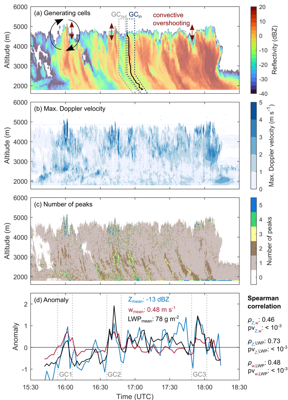
Figure 8. Time series of the radar reflectivity (a), maximum Doppler velocity (b) and number of peaks (c). The black line in panel (a) shows the 17:00 UTC fallstreak, and the dashed lines indicate the regions inside ( GC_{in} ) and outside ( GC_{out} ) of the 17:00 UTC fallstreak which were used for the analysis in Fig. 9. The maximum Doppler velocity was derived from the Doppler spectra (see Appendix A). The number of peaks were obtained from the peakTree analysis (see Sect. 2.3.2). The evolution of the cloud top anomalies is shown in (d). The radar reflectivity (blue line) and spectral width (red line) were averaged over 600 m from the cloud top. The anomalies were normalized to the mean value, which is indicated in panel (d). The results of the Spearman's rank correlation are shown to the right of panel (d), with \rho indicating the correlation coefficient and p_v the p value of the Spearman's rank correlation.
