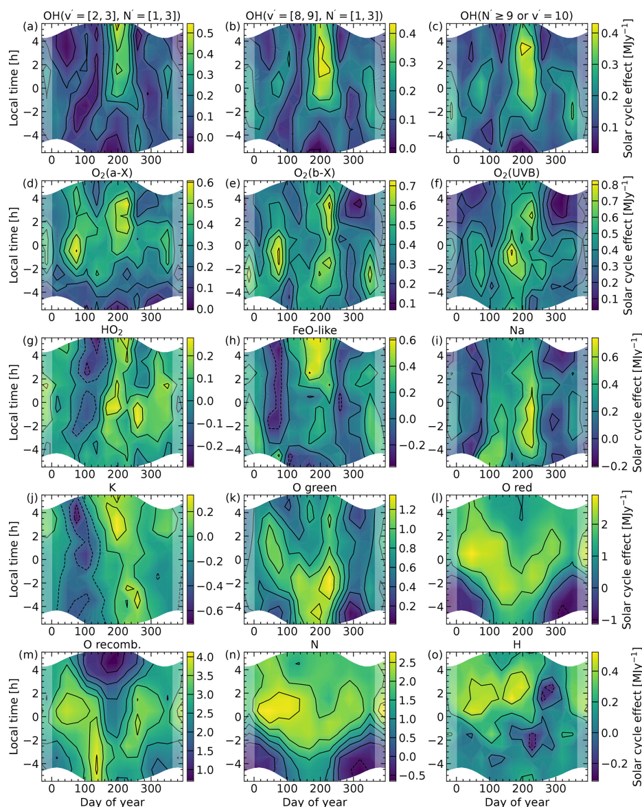
Figure 10. Climatologies of the relative intensity change by an increase in the solar radio flux of 100 sfu or 1 MJy, m_{\text{SCE}} , with respect to local time and day of year for 15 PALACE variability classes, as defined in Table 4. The solar cycle effect is provided relative to the corresponding relative intensities f_0 in Fig. 9.
