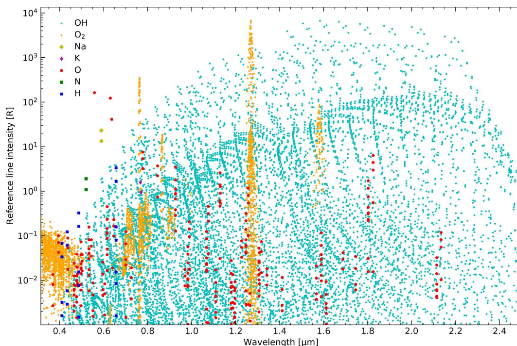
Figure 3. Reference line intensities of the PALACE model, i.e. annual nocturnal mean values for a solar radio flux of 100 sfu, as a function of wavelength. Atmospheric absorption and scattering are not applied. The 16 047 lines of OH, O 2 , Na, K, O, N, and H with a minimum intensity of 1 mR are marked by different symbols and colours (see legend).
