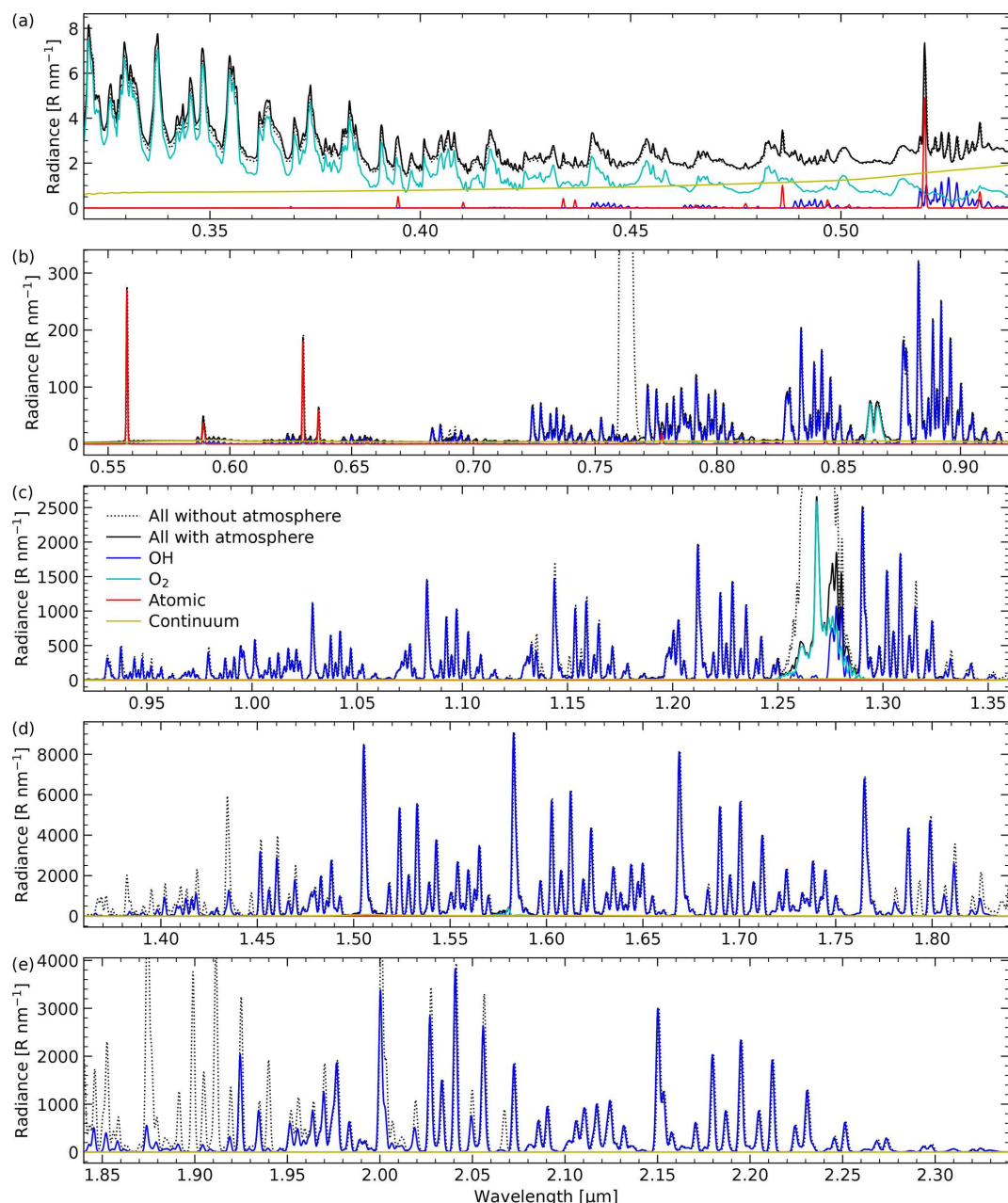
Figure 2. Reference PALACE spectrum for default model parameters provided in Table 1 in the wavelength range from 0.32 to 2.34 \mu\text{m} , divided into five sections with different radiance ranges. The combined spectrum for all components (black solid lines) is also provided without atmospheric absorption and scattering (black dotted lines). Moreover, the contributions of OH (blue), O 2 (cyan), atoms (red), and the pseudo-continuum related to HO 2 , FeO, and other molecules (yellow) are shown.
