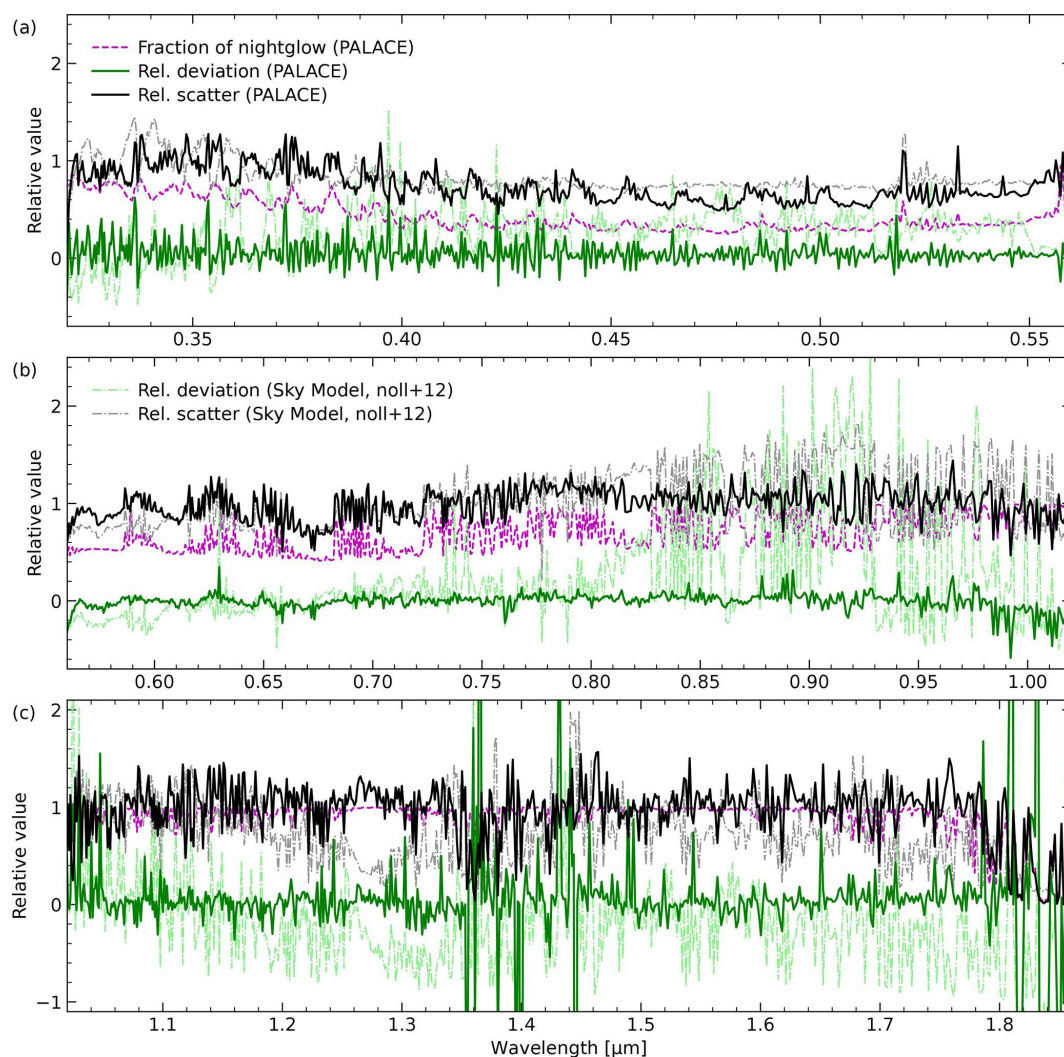
Figure 12. Evaluation of PALACE (solid lines) and the airglow component of the ESO Sky Model (Noll et al., 2012) (dash-dotted lines) based on a comparison to 6874 X-shooter spectra after the subtraction of non-airglow components calculated by means of the ESO Sky Model. Results are provided for the wavelength range from 0.32 to 1.86 \mu\text{m} , divided into three ranges related to the different X-shooter arms. The data points correspond to mean values in bins with a width of about 0.001 times the central wavelength. The green and light green curves show the mean deviation of the two models calculated for the different observing conditions from the X-shooter airglow emission relative to the average of the latter. The black and grey curves display the ratio of the mean residual variability of the models and the standard deviation of the difference between model and measured data. The dashed magenta curve indicates the average fraction of the PALACE airglow emission compared to the full sky brightness, which also considers the Sky Model non-airglow components.
