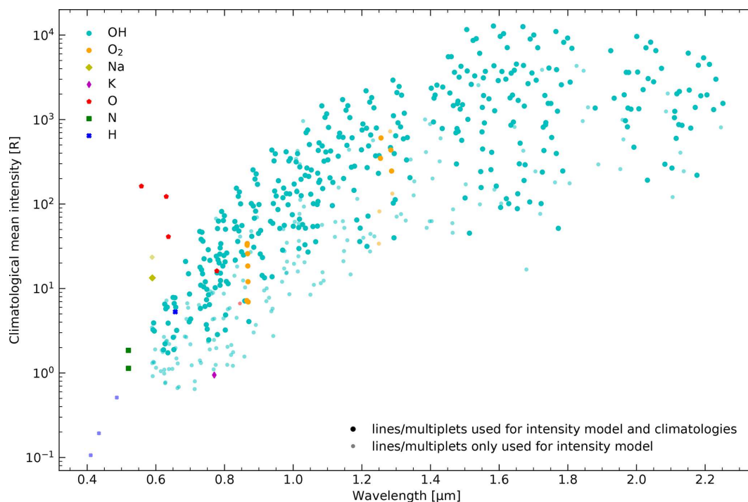
Figure 4. Individual lines or multiplets with measured climatologies that were used for the development of the mean intensity model shown in Fig. 3 (574 cases), and the derivation of the reference climatologies listed in Table 4 (392 cases, marked by big symbols; see legend). Except for the UVES-based K D 1 data from Noll et al. (2019), all data originate from X-shooter measurements. Each line or multiplet is identified by the chemical species (different symbols and colours; see legend), annual nocturnal mean intensity for 100 sfu, and wavelength.
