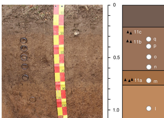
FIGURE 3 (a)–(d) Stratigraphy, position of dated charcoal (triangles/numbers, Table 2), optically stimulated luminescence samples (dots/letters, Table 3), micromorphological samples (rectangles), and standard soil parameters of soil profiles that were investigated in representative sediment traps at the four plateaus. a: Arnstein, b: Neudorf, c: Görau, d: Wallersberg. For Arnstein, horizons from augering could be correlated with those from the undisturbed soil pit despite varying absolute depths and relative thicknesses of the single horizons. Lines in redrawings mark boundaries of soil horizons. n.a.: no data available. All photos and graphics: K. Kothieringer.
