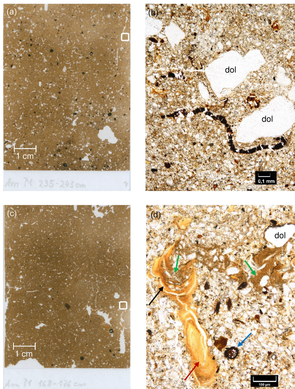
FIGURE 4 Micromorphological analysis of colluvial deposits M2 and M3 at Arnstein. (a) Scan of thin section from 2.35 to 2.43 m depth in Middle to Late Bronze Age deposit M2. Uniform, humic soil matrix, typical for colluviation. Macroscopic dark and reddish, rounded features are naturally occurring Manganese and Iron nodules. Blackish amorphous features represent plantcoal fragments. The white square marks the section shown in Figure 4b. Scan: K. Kothieringer. (b) Exemplary record of burnt root and microscopic plantcoal (black dots) in M2. Dusty silty soil matrix. Coarse fragments of dolomite (dol) rock are only weakly weathered and slightly abraded, indicating a short distance of relocation. Photomicrograph: K. Kothieringer. (c) Scan of thin section at 1.68–1.76 m depth from humic, Late Bronze Age to Middle Iron Age deposit M3. Ground mass is similar to the one of M2 due to colluviation. Plantcoal is significantly stronger fragmented and finer dispersed than in M2. The white square marks the section shown in Figure 4d. Scan: K. Kothieringer. (d) Dusty soil matrix with fragmented plantcoal and soil fungi (blue arrow), typical indicators of humic soil conditions, in M3. For explanations of the origin of bright limpid clay coatings (black arrow) and darker dusty clay and silt coatings (green arrows), see Section 4.1.2. Clay infillings (red arrow) probably developed after the decay of organic matter. Photomicrograph: K. Kothieringer.
