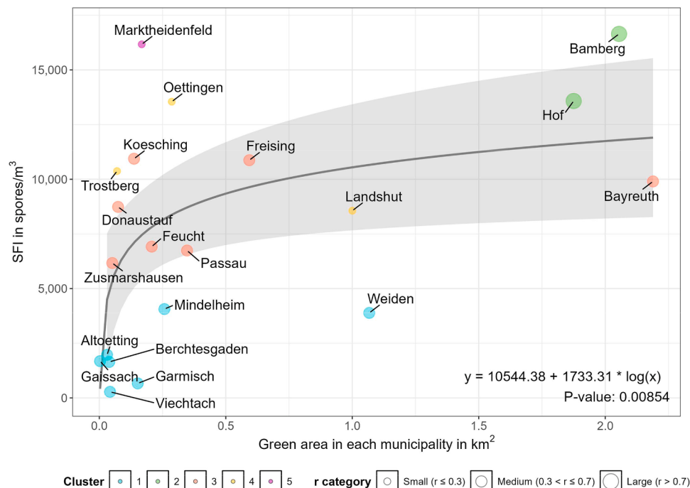
Fig. 5. Association between city green spaces and airborne Alternaria spores. Relationship between green urban areas (km 2 ) and Seasonal Fungal Index (SFI) at each location. The Munich and Augsburg sites were excluded from the analysis. Each colour represents a different cluster group identified through clustering analysis and the size of each point represents the Spearman correlation coefficient ( r ) between the green area and SFI for that location, with different sizes indicating varying strengths of the correlation.
