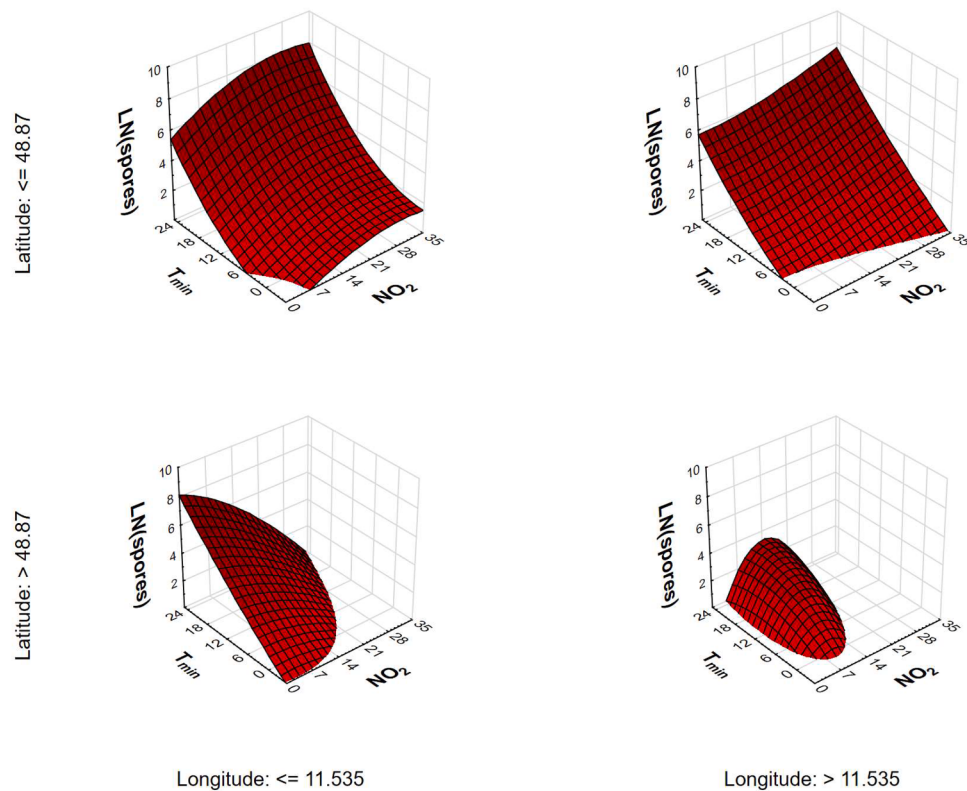
Fig. 7. Surface plot of spore concentration vs. temperature and NO 2 levels by location. Surface plot (weighted least-square difference (LSD) fitting) illustrating the logarithmic Seasonal Fungal Index (SFI) plotted against minimum temperature and NO 2 levels. The data are categorized according to four evenly distributed geographical positions, each defined by latitude and longitude coordinates.
