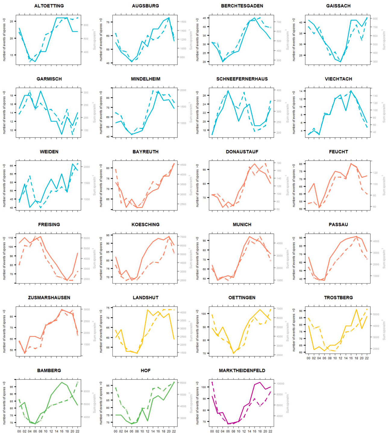
Fig. 4. Bi-Hourly spore distribution trends across sampling sites. Each panel shows the diurnal distribution of spores per sampling site during 2015 spore season (1st May to 30th September), with sites arranged alphabetically and coloured according to their cluster grouping (see Fig. 3). The X-axis displays the time of the day in 2-hours intervals (CEST, Central European Summer Time). The primary Y-axis (left in black) shows the frequency of spore occurrence for each bi-hourly interval (solid line), indicating when spores were most frequently present. The secondary Y-axis (right in grey) displays the Seasonal Spore Integral per interval (dashed line), summarising the total spore load accumulated at each time point across the season. This dual-axis approach helps distinguish between the timing and intensity of spore presence.
