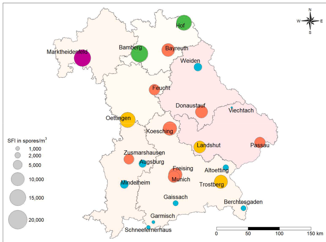
Fig. 3. Hierarchical clustering of Alternaria spore concentrations in Bavaria. Study area in Bavaria showing the results of hierarchical clustering using Ward's method applied to the complete daily Alternaria spore concentration dataset and based on temporal trends across monitoring sites. Each colour represents one of the five cluster identified in the analysis. Within each cluster, a circular marker (bubble) is displayed, with its size (see legend) proportional to the Seasonal Fungal Index (SFI) of Alternaria at each site. The legend includes representative bubble sizes for the SFI values of <5,000, <10,000, <15,000, and <20,000 spores/m 3 , allowing for a visual comparison of cumulative spore loads across regions.
