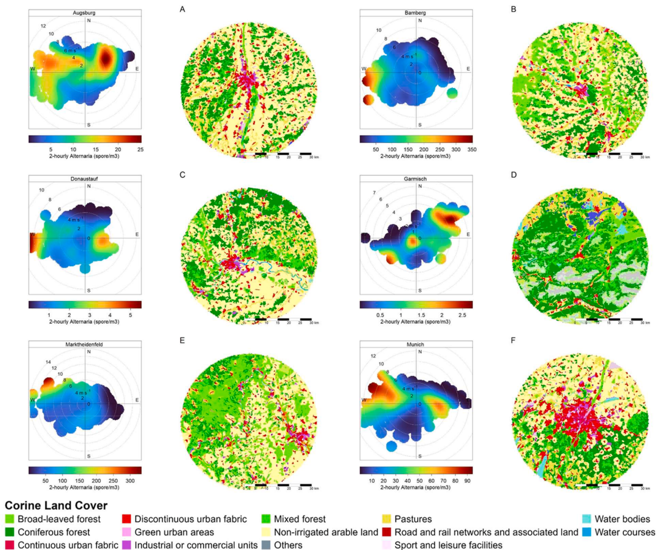
Fig. 6. Bi-hourly Alternaria concentrations in polar coordinates and site location with land cover types. Alternaria bi-hourly concentration in polar coordinates (left) showing concentration by wind speed and direction in one of the sites of each cluster and one from the Alps (Garmisch). Mean concentrations are calculated for wind speed-direction 'bins' (e.g. 0-1, 1-2 m/s and 0-10, 10-20 degrees etc.). Lower concentration of spores are in blue and the higher in red colour. On the right, the location of the spore-monitoring site and land cover types (based on Corine Land Cover data) within 30 km distance of the site. It is assumed that the amount of airborne particles recorded using volumetric trap is in general considered to reflect the overall particles load within a distance of about 30 km (Skjøth et al., 2010).
