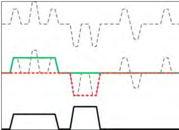
Figure 5. Top: A 1D signal composed of two textured regions and two isolated features on the right side. Middle: the green signal is an upper texture envelope; the red dashed-line signal is a lower texture envelope. Bottom: The MTC transformation. It is proportional to texture contrast and yields suppressed response at isolated features. Note that the salient feature on the top of the left texture (in the middle) is also suppressed.
