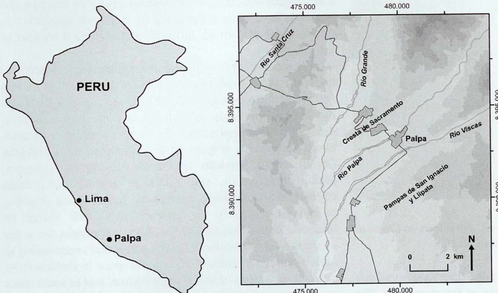
Figure 3. Palpa in the northern Nasca region on the south coast of Peru (coordinates: UTM 18S, WGS 84).
