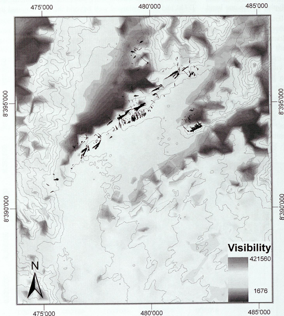
Figure 6. Interpolated visibility index of random points (blue: low visibility, red: high visibility). Geoglyphs considered in the present study are marked in black (coordinates: UTM 18S, WGS 84) (see CD-ROM for color image).
