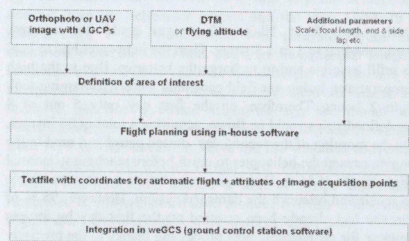
Figure 2-1: Workflow of flight planning.
