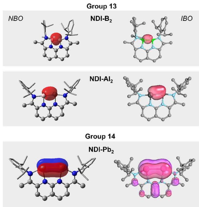
FIGURE 4 NBO (red and blue) and IBO (light red and pink) analysis of the bonding interaction between main-group element centers in E = B , Al and Pb complexes. IBO, intrinsic bond orbital; NBO, natural bond orbital.
