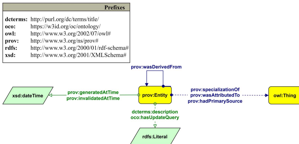
Figure 7. The Graffoo diagram describing snapshots ( prov:Entity ) of an entity (linked via prov:specializationOf ) and the related provenance information.
