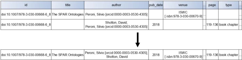
Figure 4. During a merge, the first information found takes precedence. In this example, David Shotton is inserted after Silvio Peroni in the list of authors because Peroni was already recorded as the first author, even if Shotton appears before Peroni in the second occurrence.
