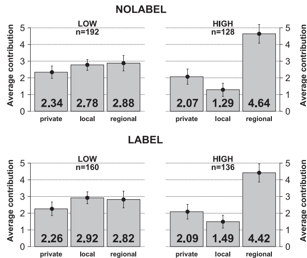
Fig. 2. Average contributions in the four treatment conditions, full sample.
