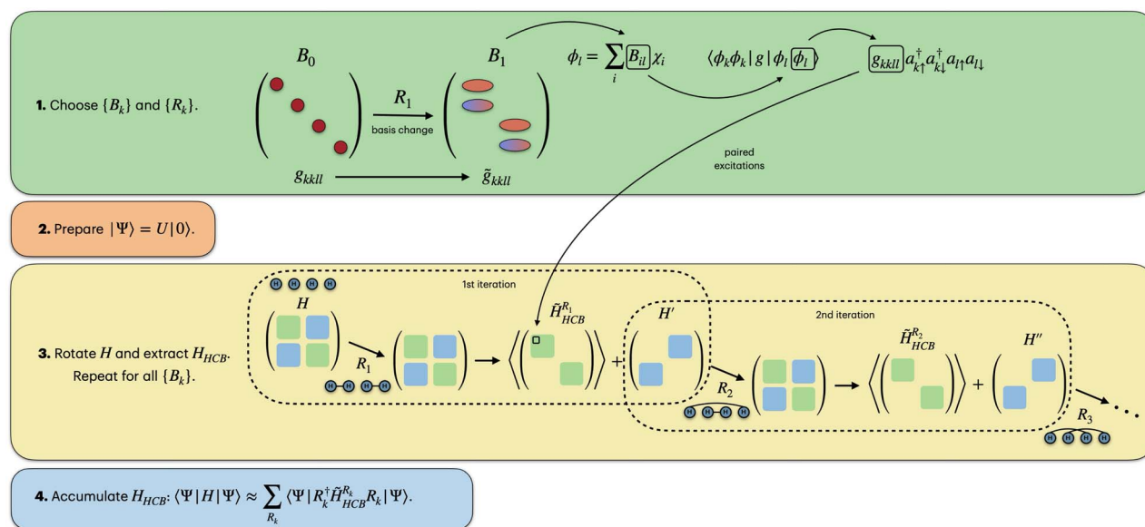
Fig. 1 Illustration of the measurement routine used in this article, leveraging the HCB approximation and basis rotations. The general procedure is applied to hydrogenic systems like H_4 (depicted in the figure), H_6 and H_8 . Here diagonal and off-diagonal matrix elements (green and blue) are used to represent HCB and residual Hamiltonian elements.
