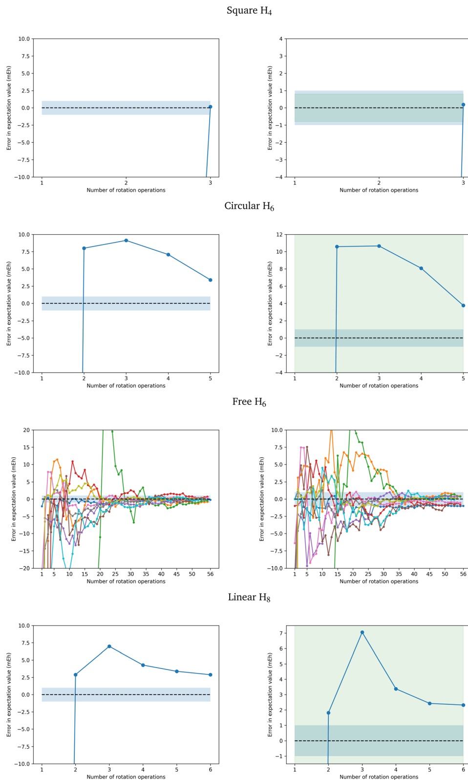
Fig. 6 Close-up visualization of Fig. 3. The blue area is the 1 mE_h margin of error, which we consider as the desired accuracy; the green area is the error from the chosen circuit ansatz.
