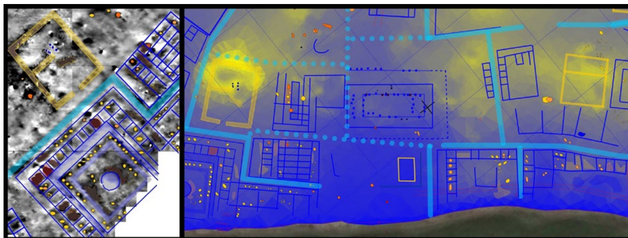
Figure 3: Details of the interpretation: macellum with high magnetic values in some tabernae (left); area of the basilica with two buildings showing as positive magnetic values (right).
