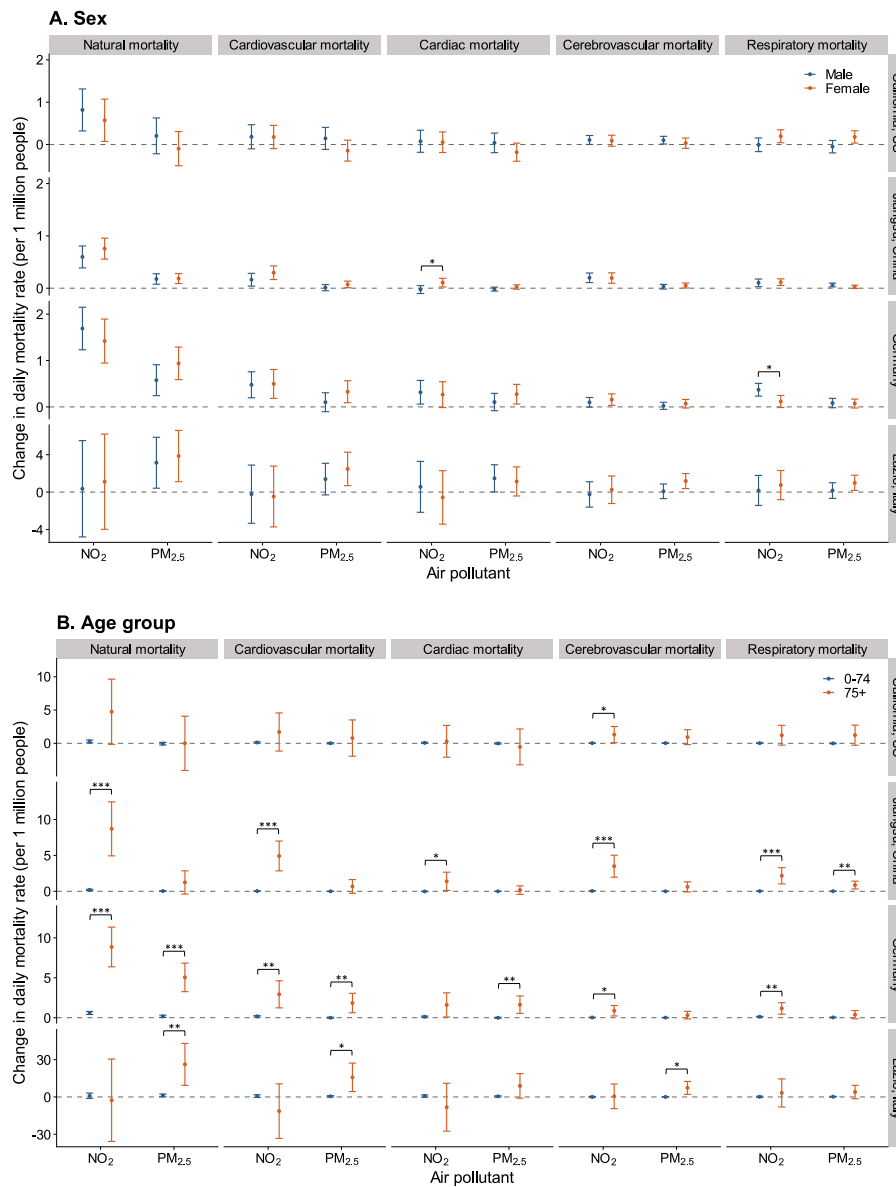
Fig. 3. Estimated change in daily cause-specific mortality rate (per 1 million people) associated with a 10 µg/m 3 increase in NO 2 or PM 2.5 concentration by effect modification.
