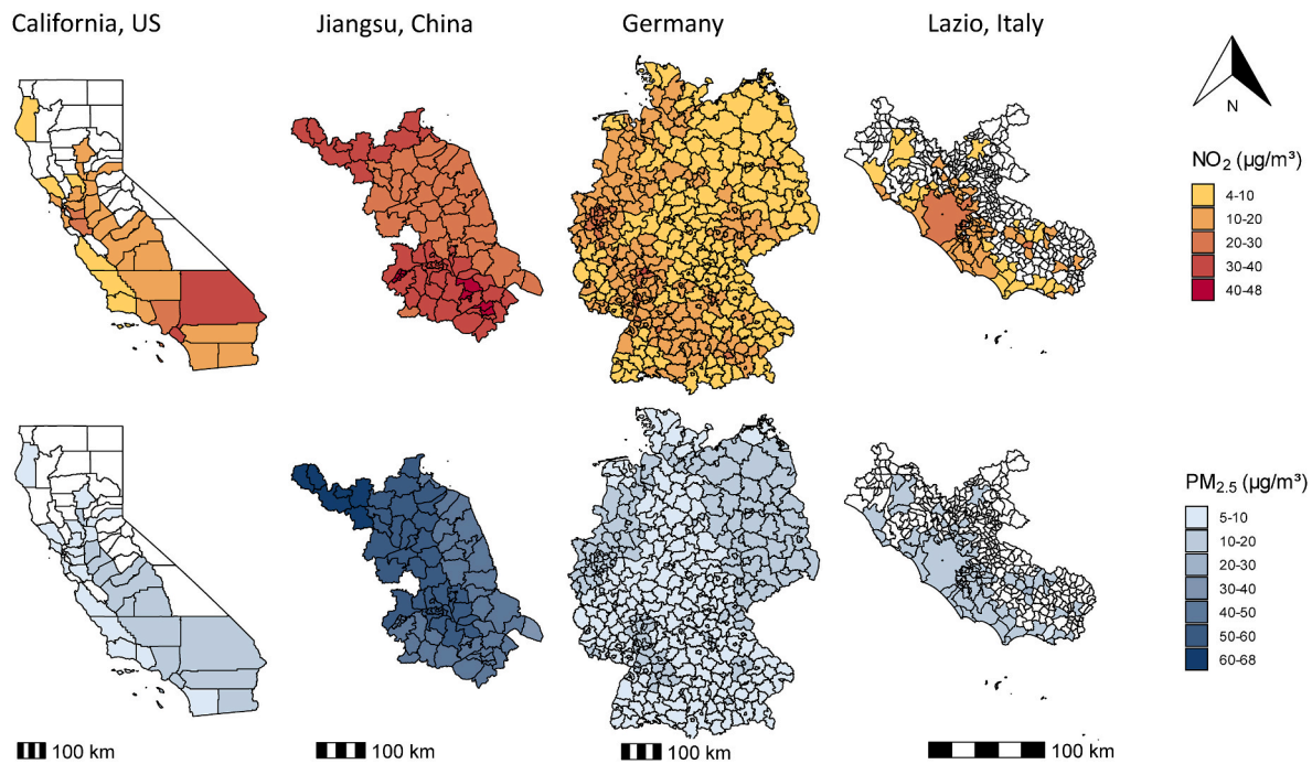
Fig. 1. Daily mean NO 2 and PM 2.5 concentrations in each spatial unit.
