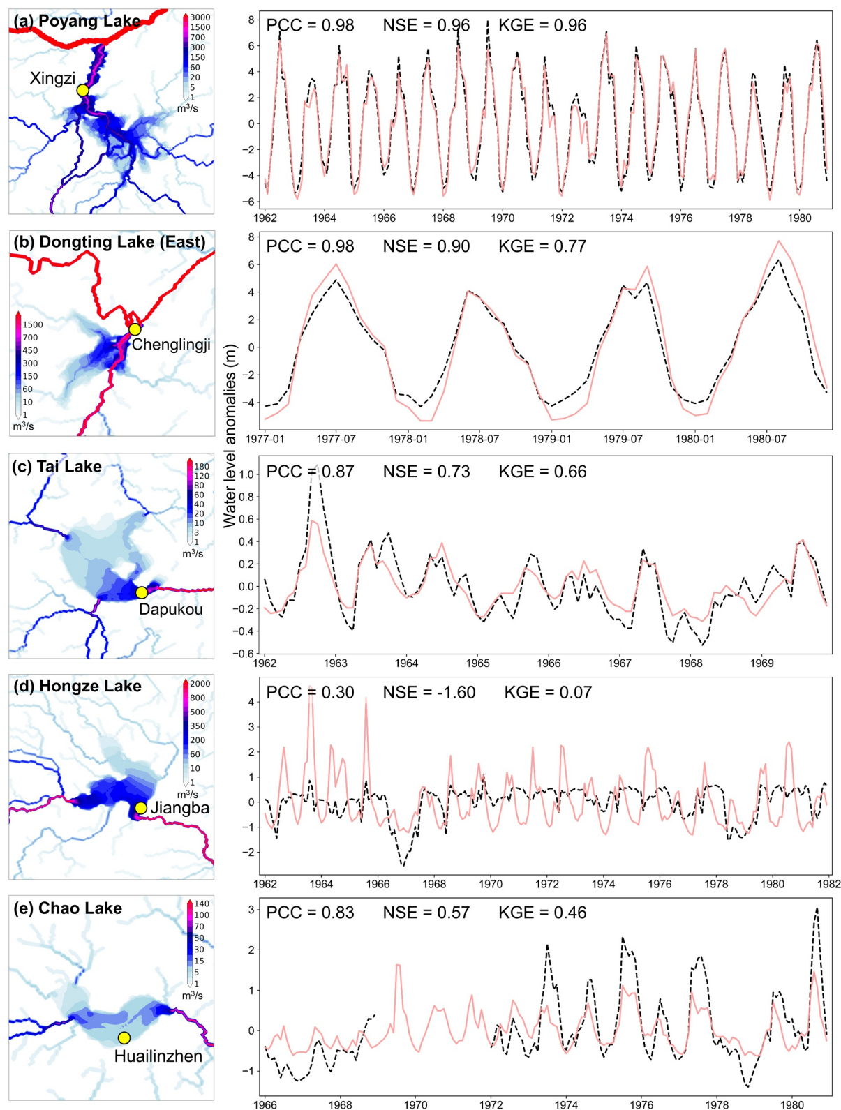
Figure 10. Simulated mean 2D flow fields across the river-lake systems of (a) Poyang Lake, (b) Dongting Lake, (c) Tai Lake, (d) Hongze Lake, and (e) Chao Lake; and the simulated monthly lake water level versus in situ observations at Xingzi, Chenglingji, Dapukou, Jiangba, and Hualinzen gauges over the same period.
